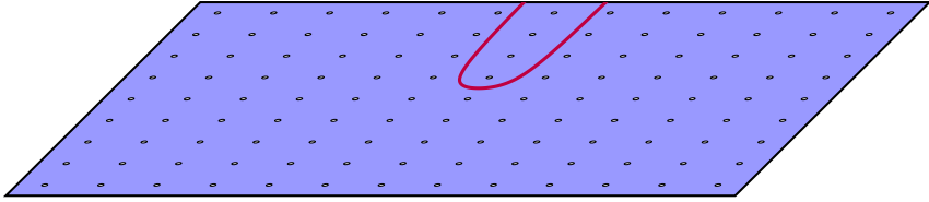
Figure 4 The half-space H in \mathbb{R}^2 \setminus \mathbb{Z}^2 .
