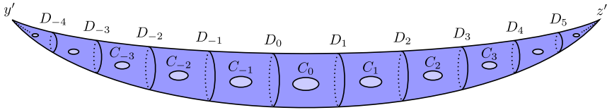
Figure 1 The surface \underline{S} .
