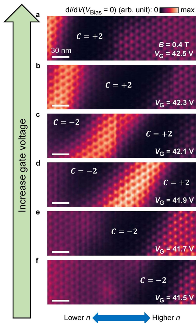
Extended Data Fig. 7 | Reversible displacement of chiral interface states via back-gating. a–f , dI/dV maps of the same area as Fig. 2a at B = 0.4 T and V_{\text{Bias}} = 0 mV for a V_G = 42.5 V, b V_G = 42.3 V, c V_G = 42.1 V, d V_G = 41.9 V, e V_G = 41.7 V, and f V_G = 41.5 V. Modulation voltage \Delta V_{\text{RMS}} = 1 mV; setpoint V_{\text{Bias}} = -300 mV, I_0 = 0.2 nA; tip height offset \Delta Z = -0.075 nm.
