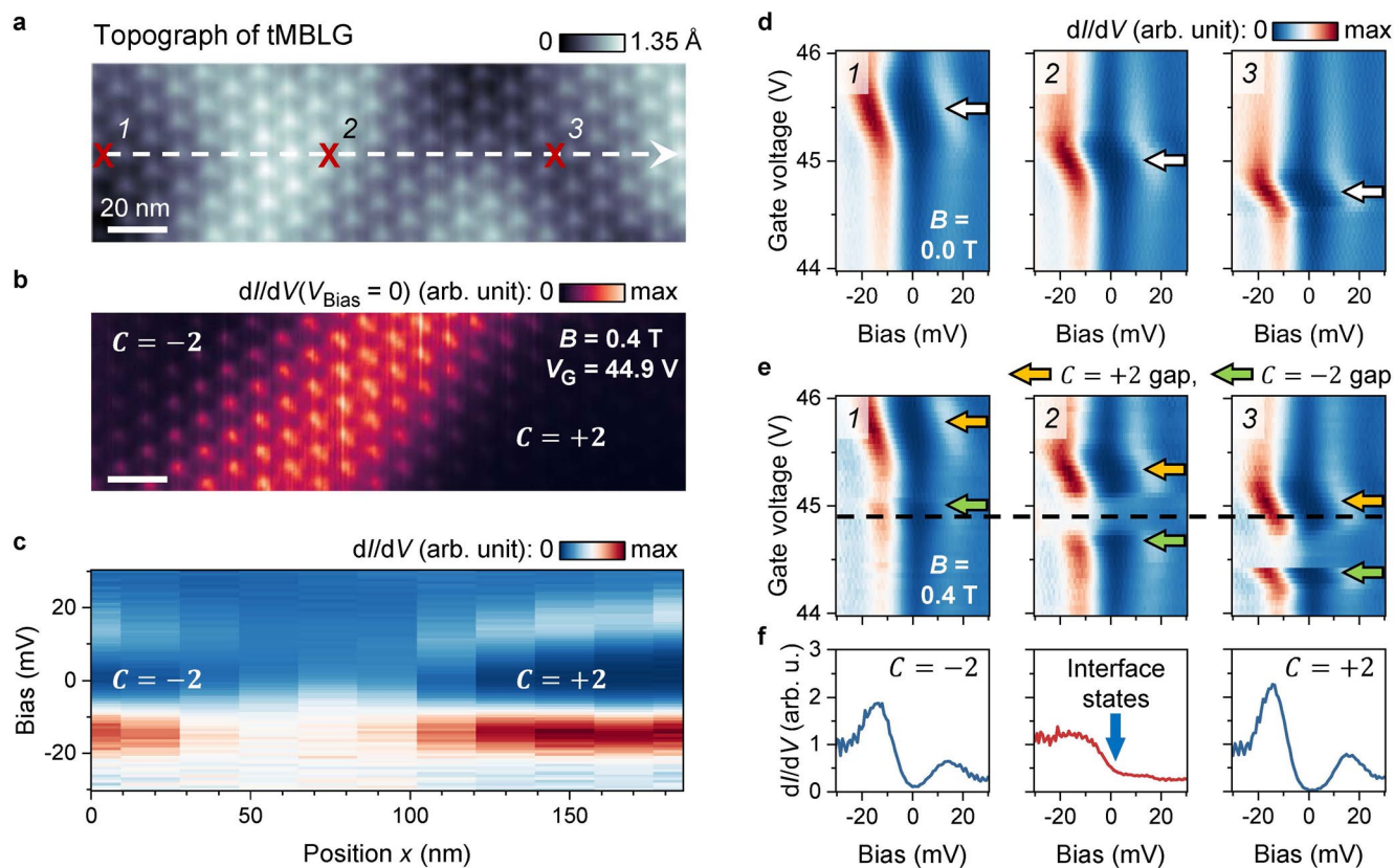
Extended Data Fig. 5 | Spatially-defined topological phase transition and chiral interface states for a different area. a , STM topographic image of a different tMBLG area ( V_{\text{Bias}} = -300 mV, setpoint I_0 = 0.2 nA). b , dI/dV map of the same area as a for B = 0.4 T, V_G = 44.9 V and V_{\text{Bias}} = 0 mV. c , dI/dV density plot for B = 0.4 T and V_G = 44.9 V obtained along the white dashed line in a . d , Gate-dependent dI/dV density plots for B = 0.0 T obtained at locations 1, 2, and 3 marked in a .
