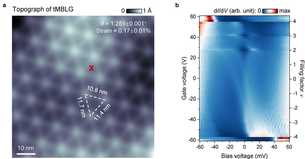
Extended Data Fig. 1 | Basic STM/STS characterization of gate-tuneable tMBLG. a , STM topographic image of a tMBLG device surface area ( V_{\text{Bias}} = -200 mV, setpoint I_0 = 2 nA). Analysis of the moiré wavelength in all three directions enables the extraction of a local twist angle of \theta = 1.251 \pm 0.001^\circ and a local hetero-strain of 0.17 \pm 0.01\% (Methods). b , Gate-dependent dI/dV density plot over the full
