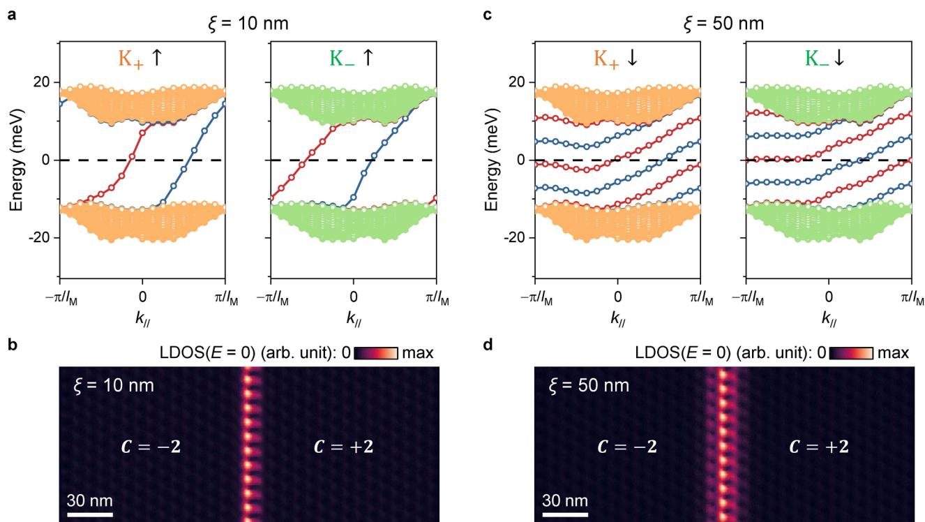
Extended Data Table. 10 | 1D band structure and chiral state image for a tMBLG Chern domain interface. a , Energy eigenvalues as a function of momentum along the interface ( k_{||} ) calculated for a Chern domain wall width of \xi = 10 \text{ nm} (the minimum value allowed in our model). Only electronic states for spin up are shown (corresponding to the sub-bands in Fig. 2h that shift upward/downward). Two branches of chiral interface states (marked by red and blue) emerge for each valley that connect the occupied and unoccupied bulk bands (thus spanning the bulk gap) and disperse unidirectionally in momentum. The total number of chiral modes (four) is equal to the Chern number difference between neighbouring domains. b , Theoretical LDOS map for E = 0 \text{ meV} showing
