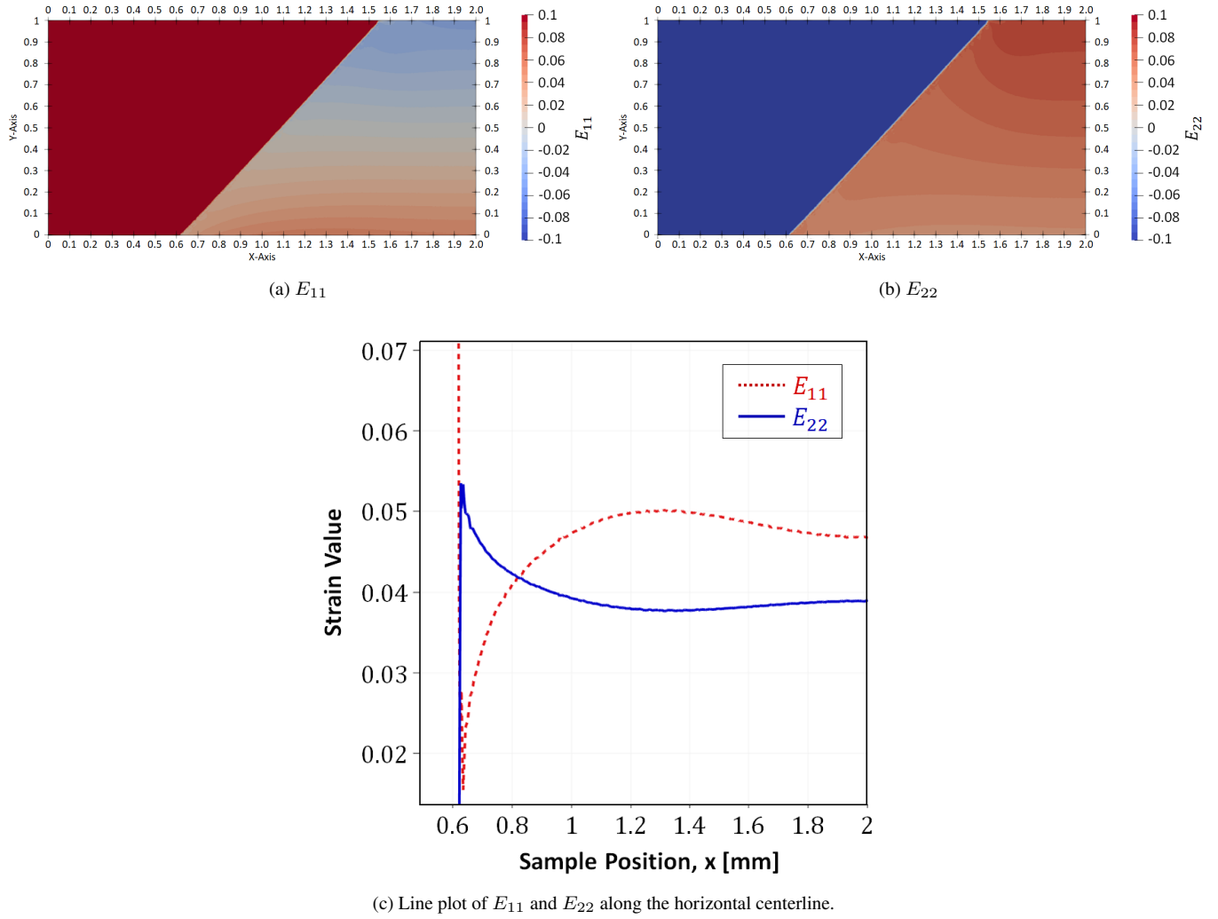
Figure 5. Plots of E_{11} and E_{22} at u_r = 0.18\text{mm} with a loading rate u_r(t) = (1 \times 10^3 \text{ mm s}^{-1}) t , with nucleation suppressed. The system reaches nonphysical regimes in the energy landscape, i.e., the strain and \phi are not consistent with Figure 2, and this would drive nucleation.
