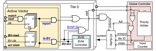
Figure 9. The control logic of a BVAP array.
