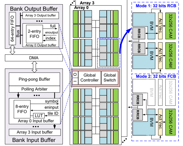
Figure 8. Overview of a hierarchical BVAP bank.
