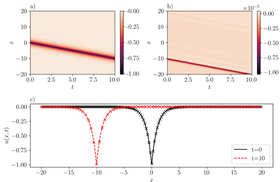
Figure 4. Same as Figure 3 but for an one-antipeakon solution in the CH equation ( b = 2 ) with c = -1 . (a): \bar{u}(x, t) inferred by SGNN; (b): error e(x, t) = u(x, t) - \bar{u}(x, t) ; (c): \bar{u}(x, t) at two time instants. In (c), “x” represents the exact solution while lines represent the prediction by SGNN. The training loss is 1.94e-11 , with \lambda_{ic} = 1000, \lambda_{bc} = 1 . Validation error: \|e\|_{\infty} = 1.02e-5, \|e\|_2 = 9.59e-13 .
