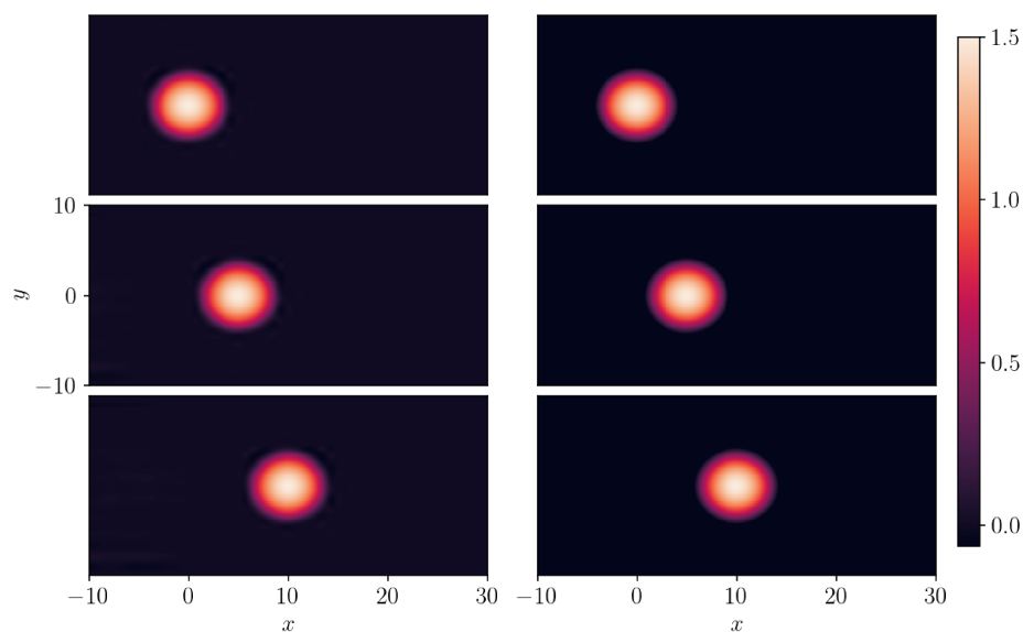
Figure 15. Same as Figure 14 but for the 2D compacton C_2(2, 0 + 3) of Equation (24) with \lambda = 1 . Left panel: SGNN prediction; right panel: ground truth. Top panel: t = 0 ; middle panel: t = 5 , bottom panel: t = 10 . The training loss: 1.23e - 3 ; \lambda_{ic} = 100 , \lambda_{bc} = 10 . Validation error: \|e\|_\infty = 0.135 , \|e\|_2 = 8.28e - 5 .
