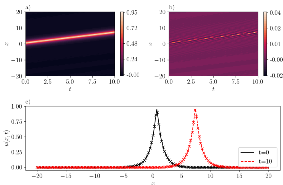
Figure 12. A peakon in the ab -family with b = 2.0, a = 1/3 . The wave speed is c = 1 . (a): \bar{u}(x, t) inferred by SGNN; (b) e(x, t) = u(x, t) - \bar{u}(x, t) ; (c) u(x, t) at two time instants. In (c), “x” markers represent the exact solution while lines depict the prediction by SGNN. The training loss is 0.0141, with \lambda_{ic} = 1000, \lambda_{bc} = 100 . Validation loss: \|e\|_\infty = 3.70e - 2, \|e\|_2 = 8.63e - 6 .
