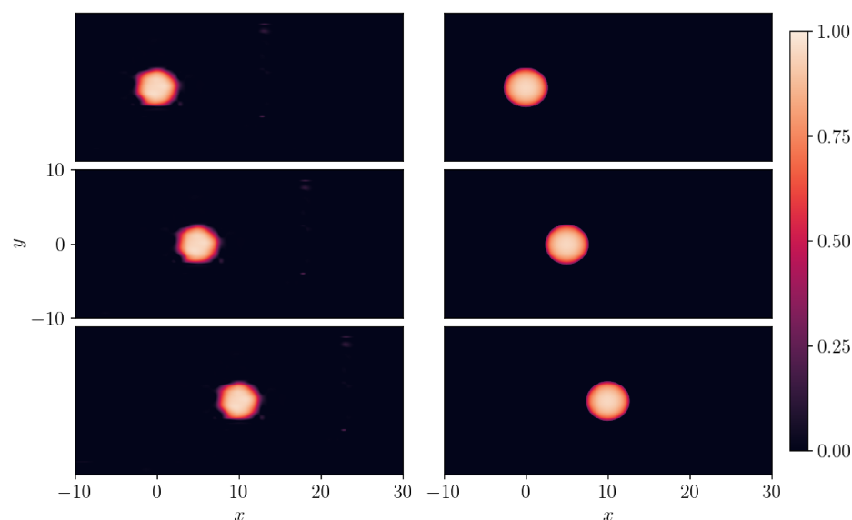
Figure 14. A 2D compacton C_2(3, 1 + 2) of Equation (22) with \lambda = 1 . Left panel: SGNN prediction; right panel: ground truth. Top panel: t = 0 ; middle panel: t = 5 ; bottom panel: t = 10 . The training loss: 9.97e - 3 ; \lambda_{ic} = 100 , \lambda_{bc} = 10 . Validation error: \|e\|_\infty = 0.371 , \|e\|_2 = 1.58e - 4 .
