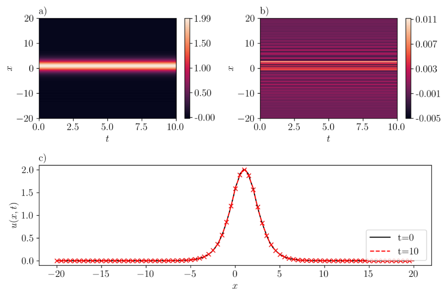
Figure 11. Same as Figure 10 but for a stationary solution, i.e., “lefton” of the b -family with b = -2.0 . (a): \bar{u}(x, t) inferred by SGNN; (b): e(x, t) = u(x, t) - \bar{u}(x, t) ; (c) u(x, t) at two time instants. The format of panel (c) is the same as the one in Figure 9. The training loss is 0.054 , with \lambda_{ic} = 1,000 , \lambda_{bc} = 1 . Validation loss: \|e\|_\infty = 1.12e - 2 , \|e\|_2 = 4.62e - 6 .
