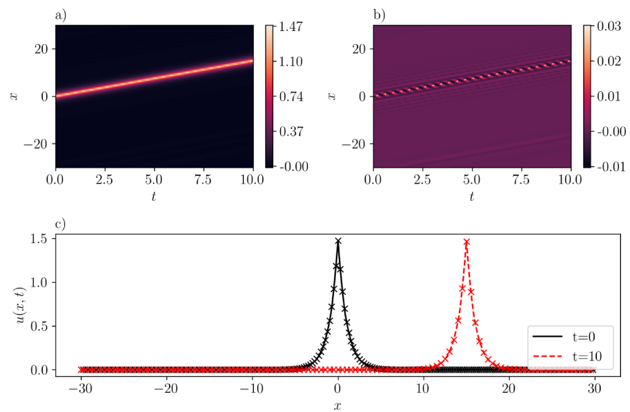
Figure 5. Same as Figure 4 but for a one-peakon solution of the b -family with b = 0.8 and c = 1.5 . (a): \bar{u}(x, t) inferred by SGNN; (b): error e(x, t) = u(x, t) - \bar{u}(x, t) ; (c): \bar{u}(x, t) at two time instants. In (c), “x” represents the analytical solution while curves represent the prediction by SGNN. The training loss is 9.18e - 2 , with \lambda_{ic} = 1000 , \lambda_{bc} = 1 . Validation error: \|e\|_{\infty} = 2.74e - 2 , \|e\|_2 = 4.09e - 6 .
