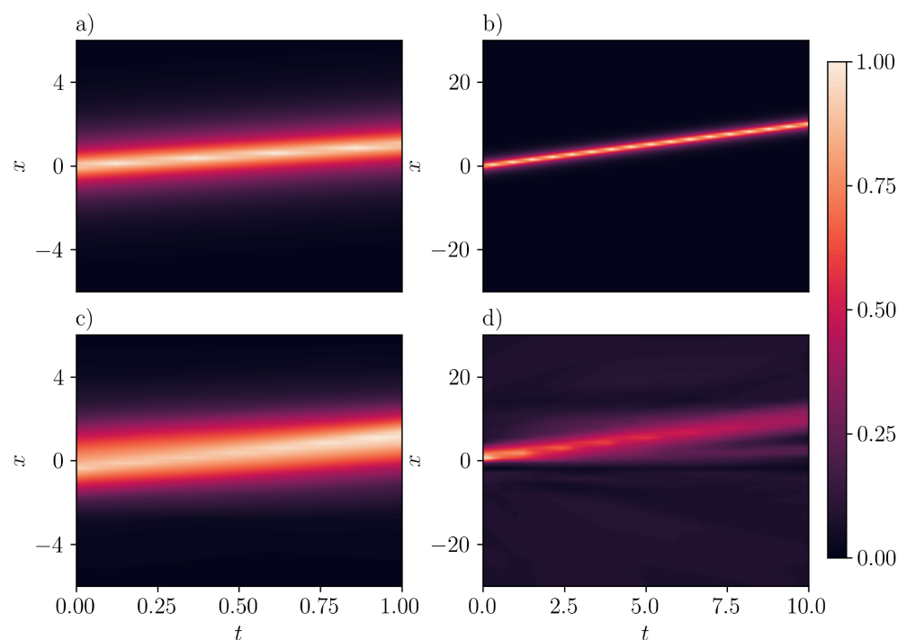
Figure 1. Inference of the spatio-temporal evolution of a peakon in the Camassa-Holm (CH) equation by PINNs. Panels (a,b) correspond to ground truth, whereas panels (c,d) to the NN approximation. For small domains, e.g., [-5, 5] \times [0, 1] (panel (c)), PINNs are able to roughly capture the correct solution. However, the propagation failure of PINNs occurs when a large spatio-temporal domain, e.g., [-30, 30] \times [0, 10] is utilized, see, panel (d). In this case, PINNs converge to a trivial solution.
