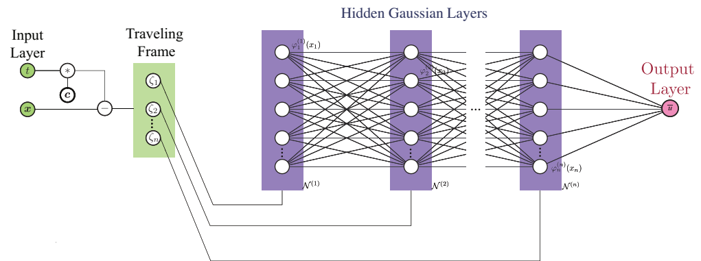
Figure 2. The architecture of SGNN with input transformed into the co-traveling frame whose coordinates (in vector form) are \zeta = \mathbf{x} - \mathbf{c}t , where \mathbf{c} represents the velocity of the wave. Different from multi-layer perceptron (MLP), the transformed input is then split and fed sequentially to hidden layers of an SGNN that consist of univariate functions. The multiplication and addition of such univariate functions in feedforward propagation can eventually lead to the summation of a set of multivariate functions used to approximate the solution of a PDE.
