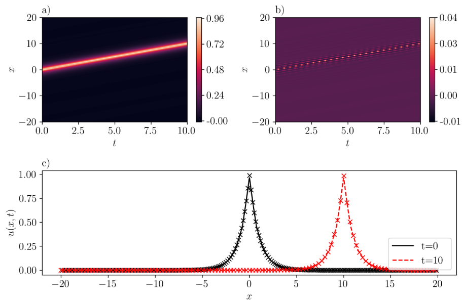
Figure 3. A one-peakon solution in the CH equation ( b = 2 ) with c = 1 . (a): \bar{u}(x, t) inferred by SGNN; (b): error e(x, t) = u(x, t) - \bar{u}(x, t) ; (c): \bar{u}(x, t) at two time instants. In (c), “x” markers represent the exact solution while lines represent the prediction by SGNN. The training loss is 8.43e-3 , with \lambda_{ic} = 1000, \lambda_{bc} = 1 . Validation error: \|e\|_{\infty} = 3.90e-2, \|e\|_2 = 7.21e-6 .
