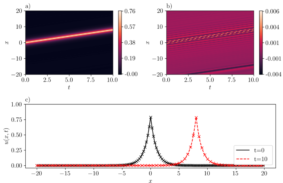
Figure 6. Same as Figure 5 but with b = -1.0 and c = 0.8 . (a): \bar{u}(x, t) inferred by SGNN; (b): error e(x, t) = u(x, t) - \bar{u}(x, t) ; (c): \bar{u}(x, t) at two time instants. The format in panel (c) is the same as in panel (c) of Figure 5. Here, the training loss is 3.10e - 2 , with \lambda_{ic} = 10,000 , and \lambda_{bc} = 1 . Validation error: \|e\|_{\infty} = 5.92e - 3 , \|e\|_2 = 3.50e - 5 .
