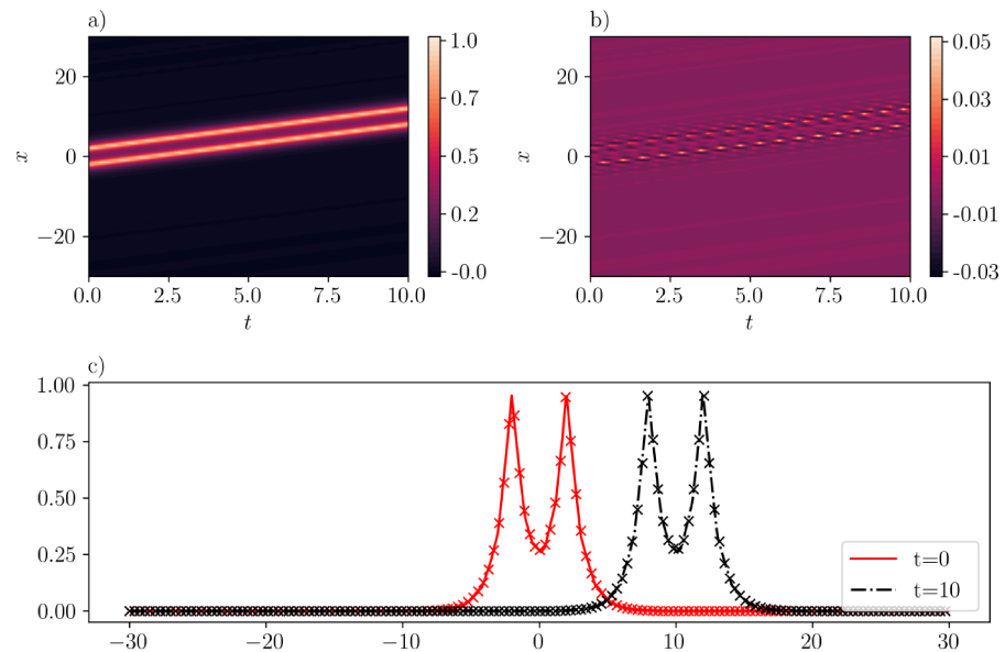
Figure 8. Two peakons with identical traveling speed ( c = 1 ) in the CH equation. (a): \bar{u}(x, t) inferred by SGNN; (b): error e(x, t) = u(x, t) - \bar{u}(x, t) ; (c): \bar{u}(x, t) at two time instants. In (c), “x” represents the exact solution while lines represent the prediction by SGNN. The training loss is 4.27e - 3 , with \lambda_{ic} = \lambda_{bc} = 100 . Validation error: \|e\|_{\infty} = 5.22e - 2 , \|e\|_2 = 2.99e - 5 .
