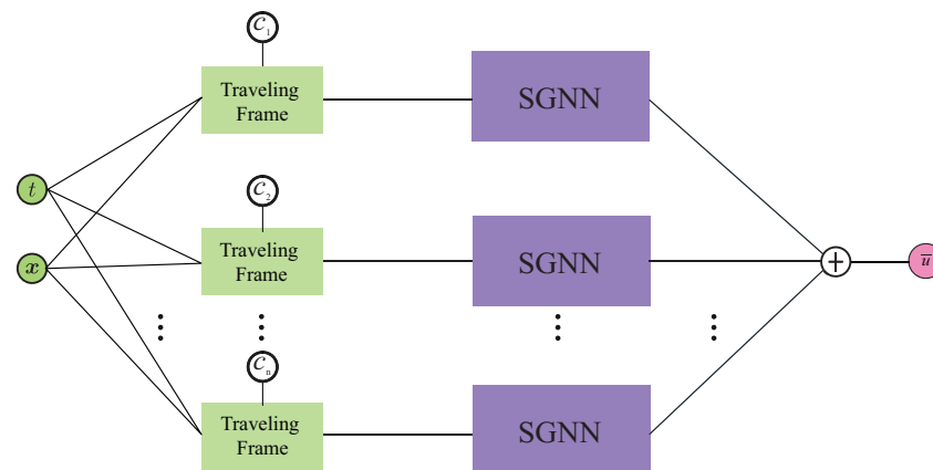
Figure 7. The NN architecture used for the study of multi-peakon configurations.
