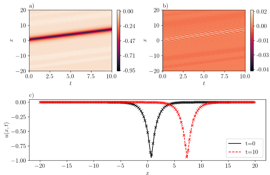
Figure 13. Same as in Figure 12, but for an anti-peakon in the ab -family with b = 2.0 , a = 1/3 , and wave speed c = -1 . (a): \bar{u}(x, t) inferred by SGNN; (b) e(x, t) = u(x, t) - \bar{u}(x, t) ; (c) u(x, t) at two time instants. The format of panel (c) is the same as the one in Figure 12. Here, the training loss is 0.0138, with \lambda_{ic} = 1000 , \lambda_{bc} = 100 . Validation error: \|e\|_{\infty} = 4.05e-2 , \|e\|_2 = 8.24e-6 .
