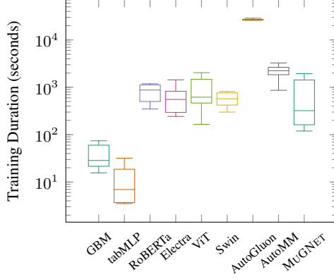
Figure 5: Training duration on all datasets.
