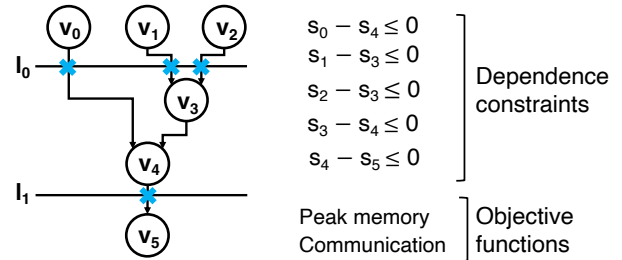
Figure 1: Example of SDC-based scheduling — (left) A DAG with two schedule stages l_0 and l_1 with latency L = 3 ; (right) Dependence constraints and objective functions including peak memory minimization and inter-stage communication minimization (the blue crosses)
