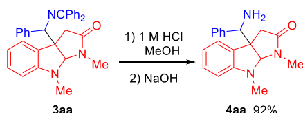
Scheme 2 (a) Gram-scale sequential one-pot synthesis. (b) Hydrolysis of the product imine.
