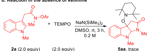
Scheme 3 Control experiments. (a) Radical trapping experiment. (b) Reaction in the absence of ketimine.
