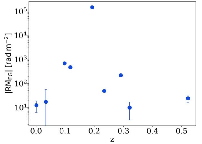
Figure 3. Amplitude of the extragalactic rotation measure ( |\text{RM}_{\text{EG}}| ) as a function of redshift ( z ) for the full set of FRBs in this sample. Error bars are shown, where some errors are smaller than the points. There is no significant correlation between the two, in sharp contrast to the burst DM, which shows a clear dependence on redshift (evidenced in the Macquart relation; Macquart et al. 2020; James et al. 2022). This indicates no strong influence from intergalactic magnetic fields and that the local environment (host and immediate burst environment) dominates |\text{RM}_{\text{EG}}| . The extremum of the |\text{RM}_{\text{EG}}| distribution is FRB 20121102A, which is expected to reflect a highly magnetized environment in which the burst resides.
