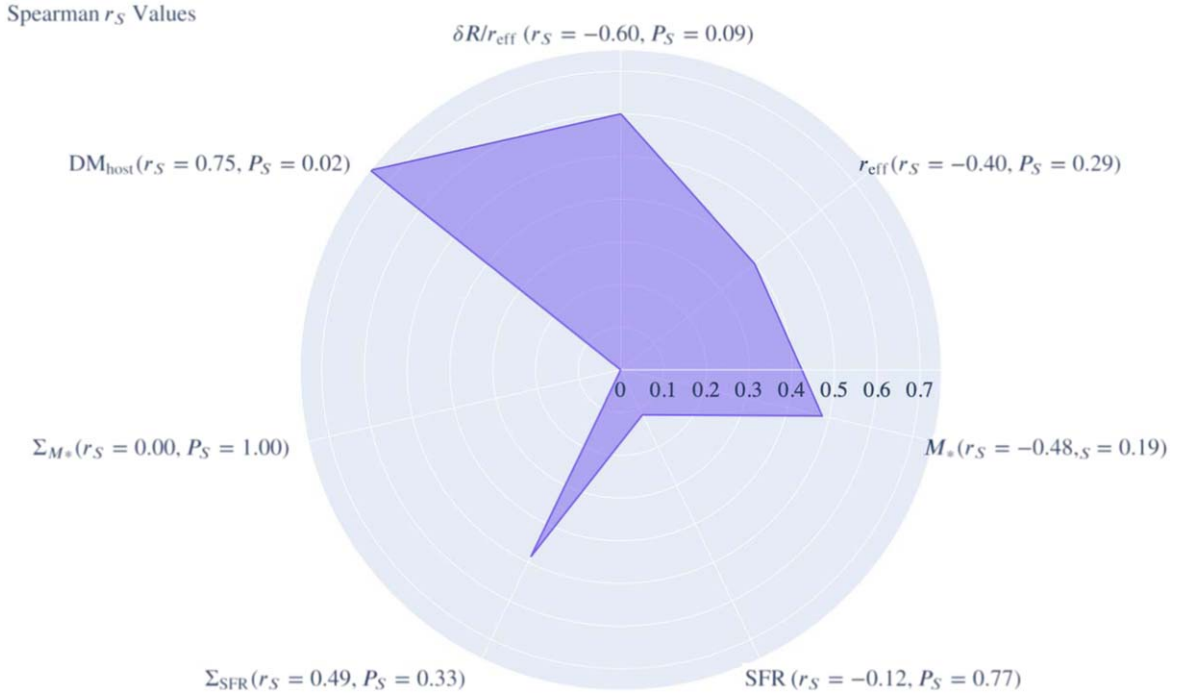
Figure 4. A radar plot showing Spearman r_S values as tests for the correlation between absolute rotation measure ( |RM| ) and a range of galaxy-scale and local-environment-related measures. The radial values represent the absolute value of the stated r_S values, and the associated significance measures are shown as well. A negative r_S represents anticorrelation. The only correlation meeting our significance criterion ( P_S < 0.05 ) is that with DM_{\text{host}} . This positive correlation can naturally arise from the fact that both quantities are sensitive to the electron density in the host ISM.
