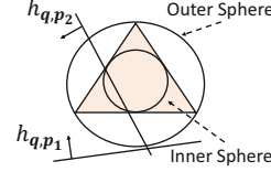
Figure 5: Relationship
