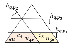
Figure 6: Sampled u
