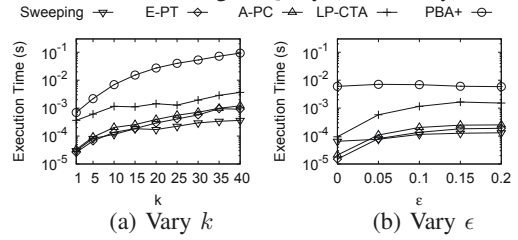
Figure 10: 2D
