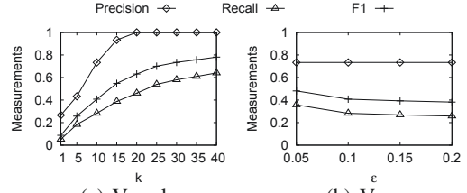
Figure 8: The Results of Reverse Top- k Query Compared with the Results of Reverse Regret Query (User Study)
