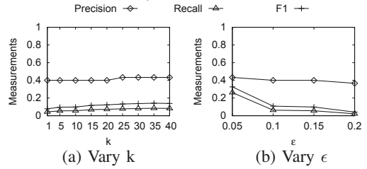
Figure 12: The Results of Reverse Top- k Query Compared with the Results of Reverse Regret Query (4D)
