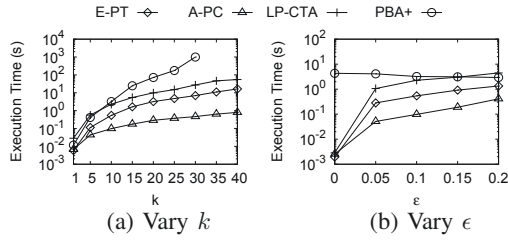
Figure 11: 4D
