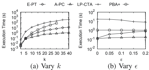
Figure 18: Weather
