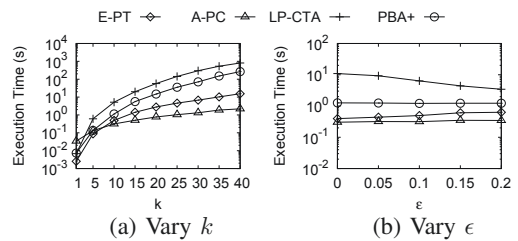
Figure 19: NBA
