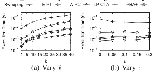
Figure 16: Island
