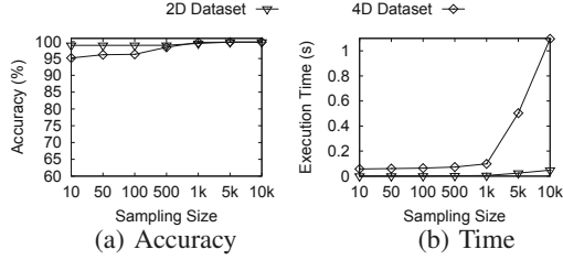
Figure 9: Accuracy
