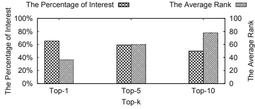
Figure 7: User Study
