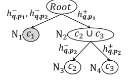
Figure 4: P-Tree
