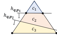
Figure 3: High Dim
