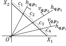
Figure 2: Two Dim
