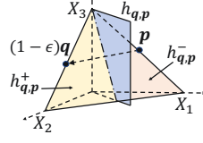
Figure 1: Hyper-plane
