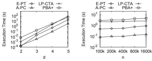
Figure 13: Vary d
