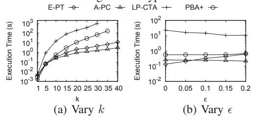
Figure 17: Car
