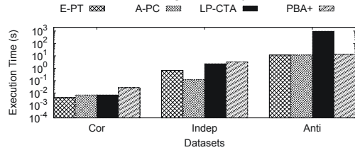
Figure 15: Type
