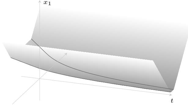
FIGURE 1. Representation of the boundary \partial C . Notice that any slice of C at a fixed t = t_0 coincides with \Sigma_\lambda for some \lambda > 0 .
