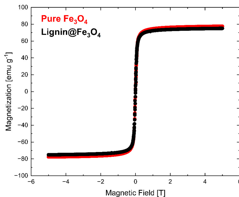
Figure 6. Magnetization measurement results (VSM) show the saturation magnetization of pure \text{Fe}_3\text{O}_4 and lignin@ \text{Fe}_3\text{O}_4 at 300 K.
