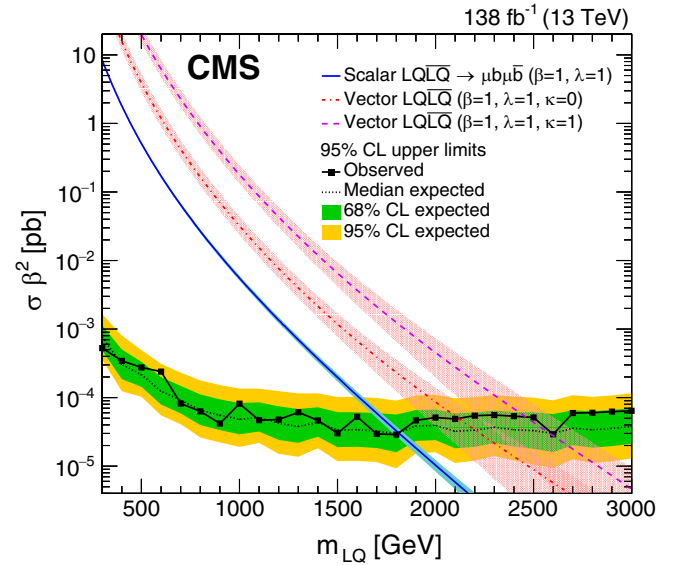
FIG. 7. The expected and observed upper limits at 95% CL on the product of the LQ pair production cross section and the branching fractions \beta^2 as a function of m_{LQ} . The black solid line represents the observed limits, the dotted line is for the median expected limits, and the inner dark-green and outer light-yellow bands are for the 68% and 95% CL intervals. The solid blue line and corresponding blue band represents the theoretical scalar LQ pair production cross sections and the uncertainties on the cross sections due to the PDF prediction and renormalization and factorization scales, respectively. Similarly, the dash-dotted (dashed) line and corresponding band represents the cross sections of theoretical vector LQ pair production and uncertainties in the minimal coupling (Yang-Mills) scenario.
