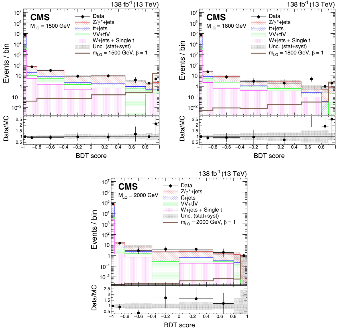
FIG. 4. Comparison of data and background BDT discriminant distributions at the preselection level for LQ mass hypotheses of 1500 GeV (upper left), 1800 GeV (upper right), and 2000 GeV (lower). The error bars are the data statistical uncertainties, while the shaded band represents the combined statistical and systematic uncertainty in the full background estimate.
