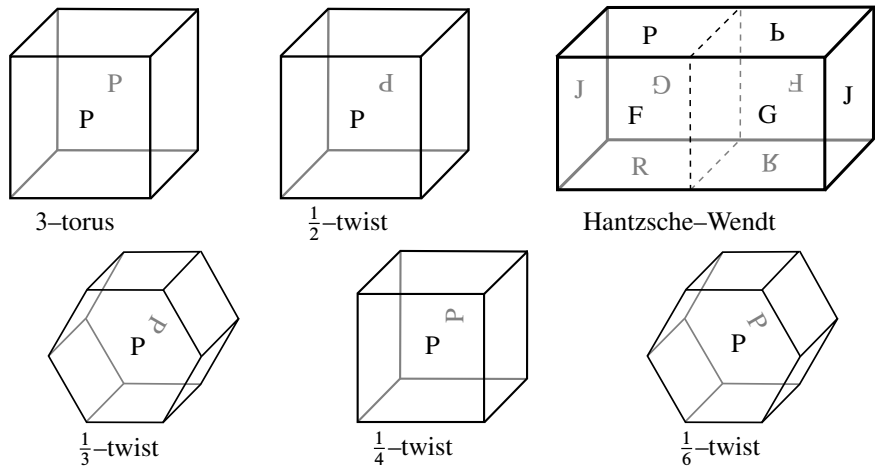
Figure 1: The fundamental domains for the manifolds in Table 1.
