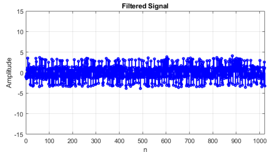
Fig. 7: Received signal after elimination of AF TD jamming signal.
