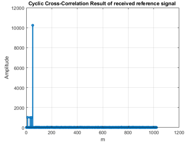
Fig. 6: Cyclic cross-correlation between the GPS receiver signal r[n] in (4) and the PN sequence p[n] versus the lag m .
