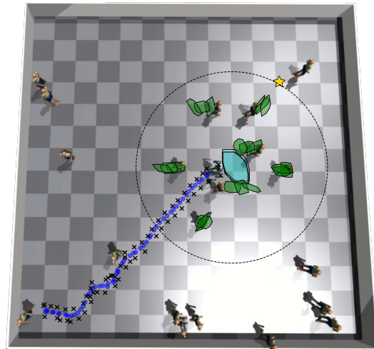
Fig. 1: Snapshot of the simulation environment with superimposed zonotopes for the proposed reachability-based social navigation framework. The environment is a 14 m \times 14 m open space with 20 pedestrians.
