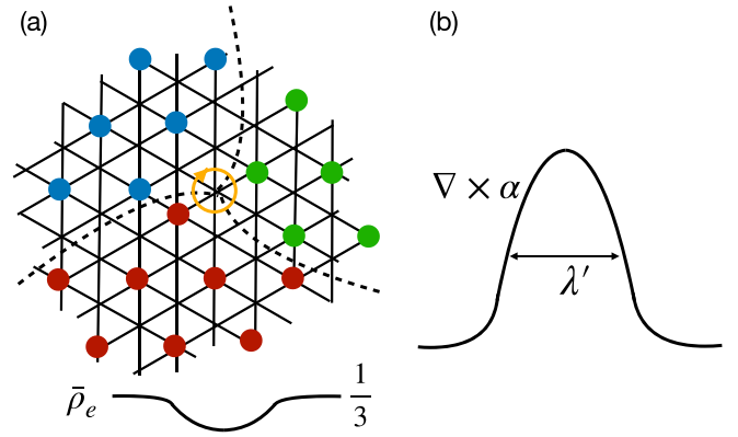
FIG. 2. (a) Drawn is the defect in the CDW ordered phase where a 1/3 charge deficit occurs. The dashed lines are the domain walls of the CDW order parameter: the orders on two sides of the wall are related by translation by one lattice constant along the domain wall direction. The charge patterns in different domains are distinguished by colors. Around the defect, the coarse-grained charge density \bar{\rho}_e will deviate from the average 1/3 in the CDW phase. A circulating current around the defect, i.e., an FQAH patch, will change the local magnetization. (b) The defect is identified as a flux of the gauge field \alpha , with a spatial extent given by the penetration depth of the vortex condensate.
