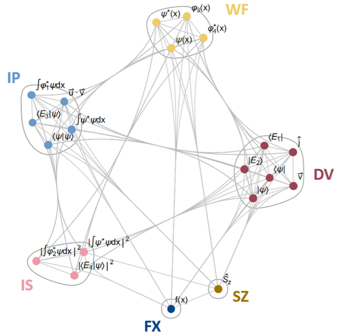
FIG. 7. The network built from student survey responses, as in Fig. 4, grouped into the six stable communities as determined by the bootstrapping procedure shown in Fig. 6. FX contains only the generic function f(x) ; SZ contains only the spin-Z operator \hat{S}_z ; DV contains Dirac bras, kets, and generic vector expressions \vec{v} and \hat{j} ; WF contains the wave function and its conjugate [ \psi(x) and \psi^*(x) ], as well as the wave function and conjugate wave function expressions for eigenstates ( \varphi_3(x) and \varphi_4^*(x) ); IP contains inner product expressions, including a generic dot product in both Dirac and wave function notation; IS contains complex squares of inner products in both notations.
