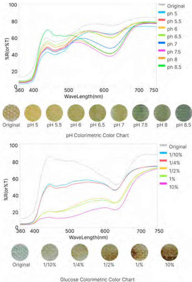
Figure 8: Colorimetric Sensing Threads Characterization
