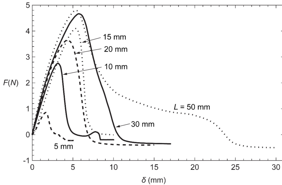
Fig. 21. Vertical force versus tip deflection from experiment for six beam lengths.
