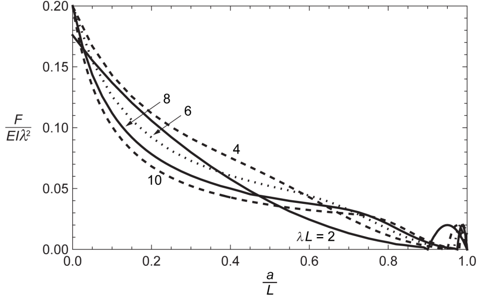
Fig. 7. Nondimensional vertical force versus nondimensional unbonded length: M_0 = 0 , a_0 = 0 , W = 0 , \gamma\lambda^2 b/k = 0.005 ; \lambda L = 2 (solid), 4 (dashed), 6 (dotted), 8 (solid), 10 (dashed).
