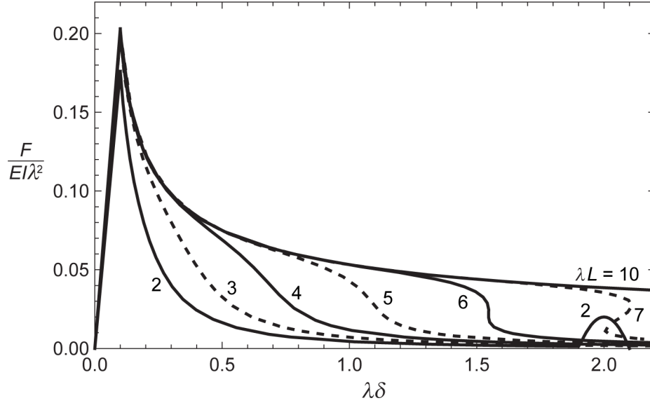
Fig. 5. Nondimensional vertical force versus nondimensional tip deflection: M_0 = 0 , a_0 = 0 , W = 0 , \gamma\lambda^2 b/k = 0.005 .
