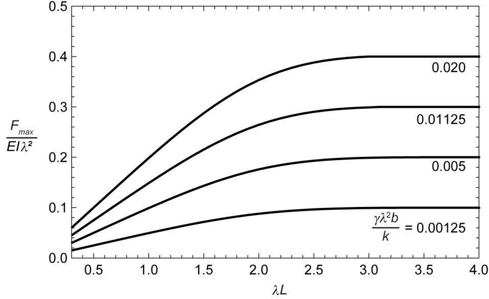
Fig. 8. Nondimensional maximum vertical force versus nondimensional beam length: M_0 = 0 , a_0 = 0 , W = 0 ; \gamma\lambda^2b/k = 0.00125, 0.005, 0.01125, 0.020 ( \lambda y_c = 0.05, 0.10, 0.15, 0.20 ).
