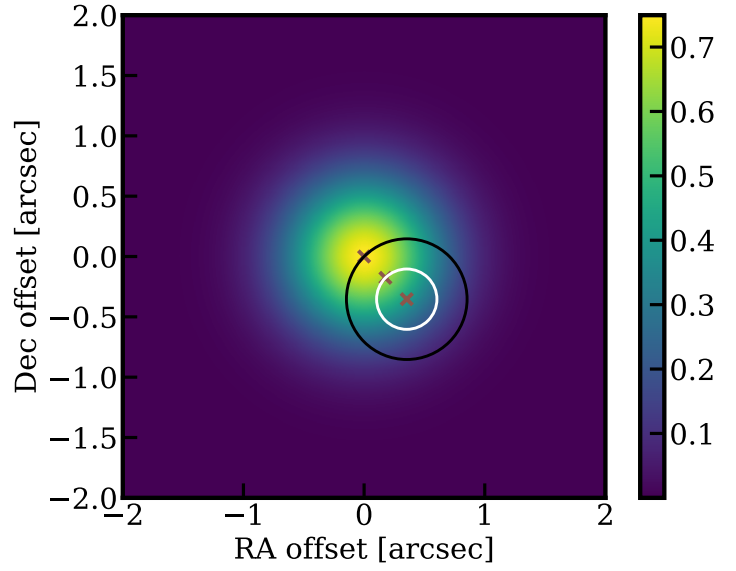
Fig. B.5: A two-dimensional Gaussian function with a total integration of one and a FWHM of 0.5'' (color scale). This is assumed as a typical emission distribution for COMs based on the results of PILS (e.g., Jørgensen et al. 2016 ). Two circular regions with radii of 0.25'' and 0.5'' are over plotted representing beams of PILS (white) and Band 3 (black), respectively. The crosses show the peak position, 0.25'' , and 0.5'' offset positions.
