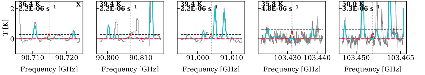
Fig. B.3: Lines of G'Gg'gg'-Glycerol and the model for its upper limit ( 7 \times 10^{15} \text{ cm}^{-2} ) in red. The symbols are the same as Fig. 3.
