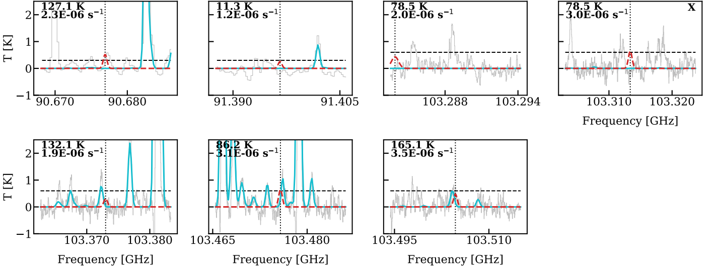
Fig. B.2: Lines of Ga-n-propanol and the model for its upper limit ( 6 \times 10^{15} \text{ cm}^{-2} ) in red. The symbols are the same as Fig. 3.
