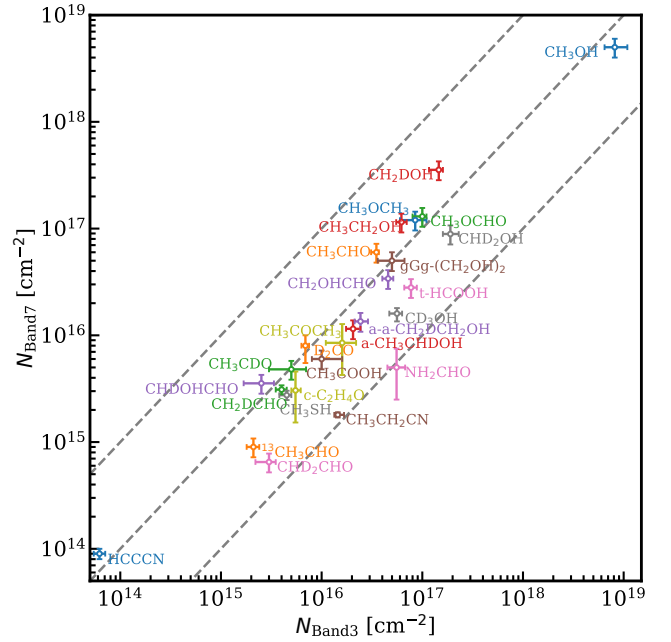
Fig. 5: Column density of the various molecules from the ALMA Band 7 observations (PILS; \sim 345 GHz) as a function of those from Band 3 ( \sim 100 GHz). Beam dilution is corrected for the column densities in this figure. Dashed lines present where the values of y-axis are the same as values of x-axis, where they are 10 times higher and 10 times lower than the values of x-axis.
