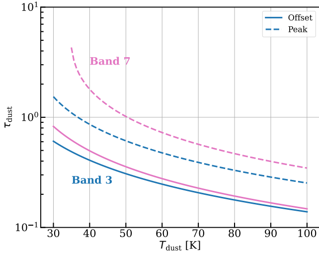
Fig. 4: Continuum optical depth as a function of temperature at the peak of the continuum (dashed) and the 0.5'' offset position where the spectrum is extracted (solid line). Blue shows the optical depth for the Band 3 continuum at frequency of \sim 91 GHz and pink shows the PILS continuum at frequency of \sim 348.815 GHz.
