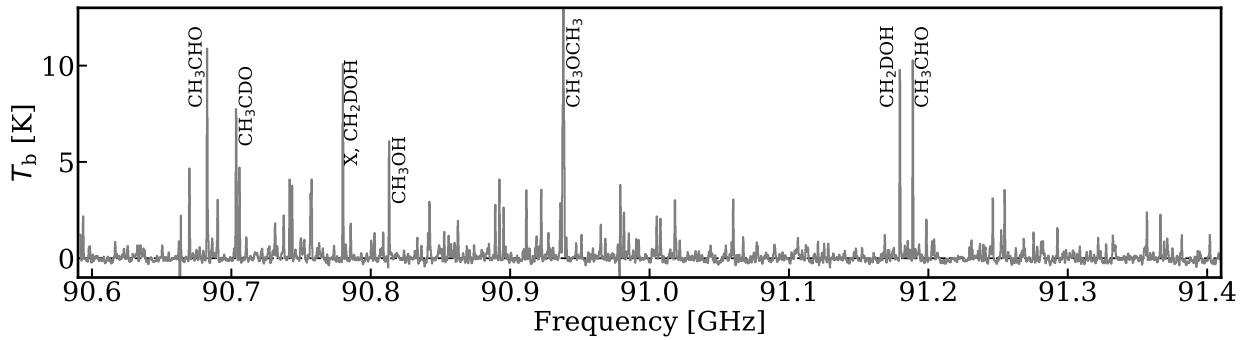
Fig. 1: The spectrum of IRAS16293 B Band 3 data for the continuum window. A few strong lines are highlighted, for the full line identification and fitting see Fig. B.1. ‘X’ indicates a line that is not yet identified and is not (fully) fitted with the considered molecules in this work. The spectrum of IRAS16293 B is line rich even at ALMA Band 3 wavelengths ( \sim 3 mm).
