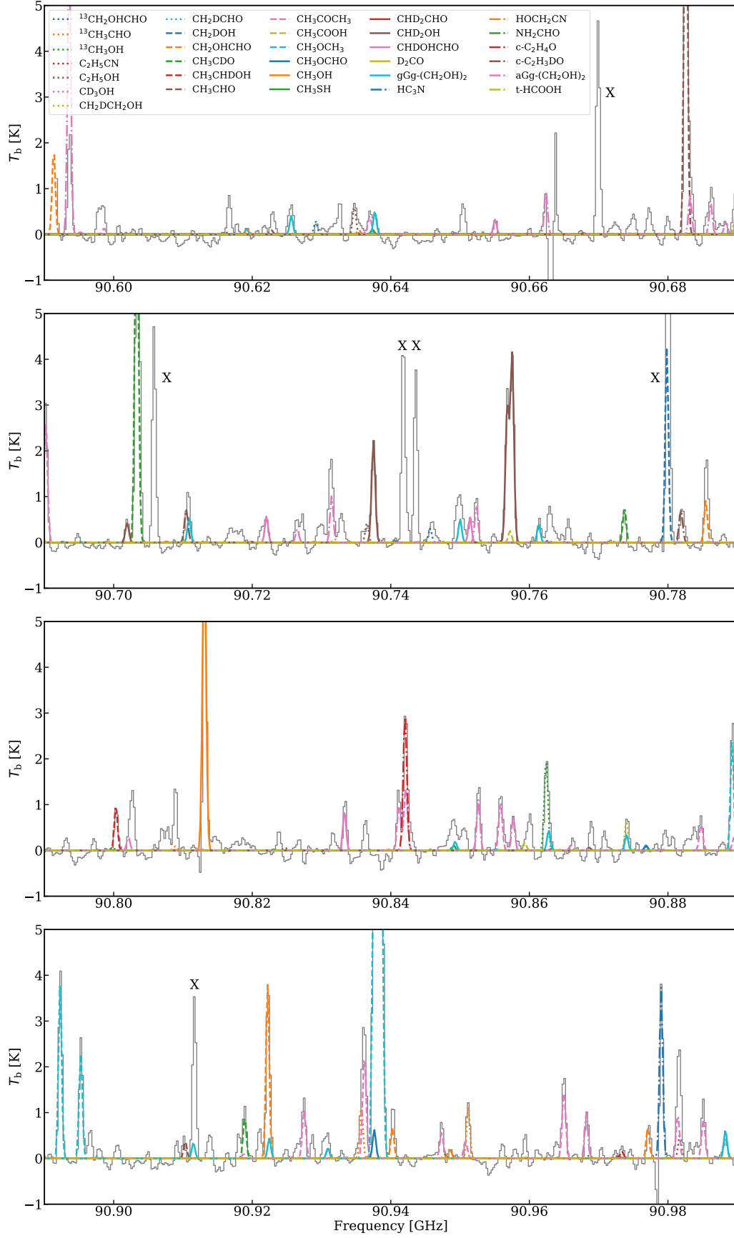
Fig. B.1: The fitted model for each molecule; on top of the Band 3 data in gray. For readability the y-axis limit is set to 5 K, however, no line is overestimated except those of methanol and one line of \text{aGg}'-(\text{CH}_2\text{OH})_2 , which are potentially optically thick. The lines that have an intensity higher than 2 K (i.e., detected at a \geq 7 - 10\sigma level), but are not identified are indicated by an 'X'.
