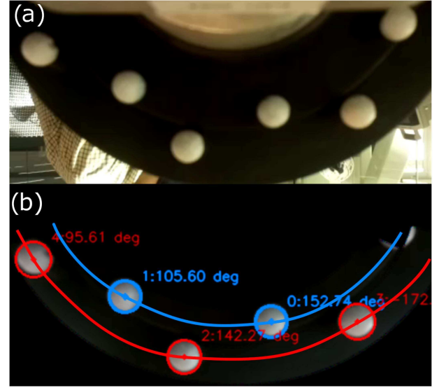
Fig. 6. Optical measurements allowed us to evaluate the true deflection of the springs. (a) High-definition video recorded the movement of the optical fiducials. (b) We tracked each fiducial within the frame, fit the tracked circles to an ellipse, and detected changes in the orientation to calculate angular position.
