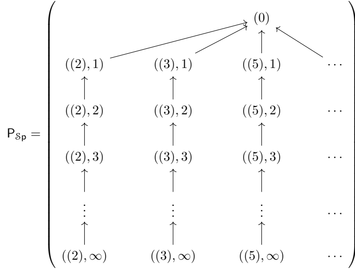
FIGURE 4. The poset P_{Sp} is the union of the totally ordered sets \{((p), \infty) \rightarrow \dots \rightarrow ((p), 2) \rightarrow ((p), 1) \rightarrow (0)\}_{p \text{ prime}} over their common maximal element (0) .
