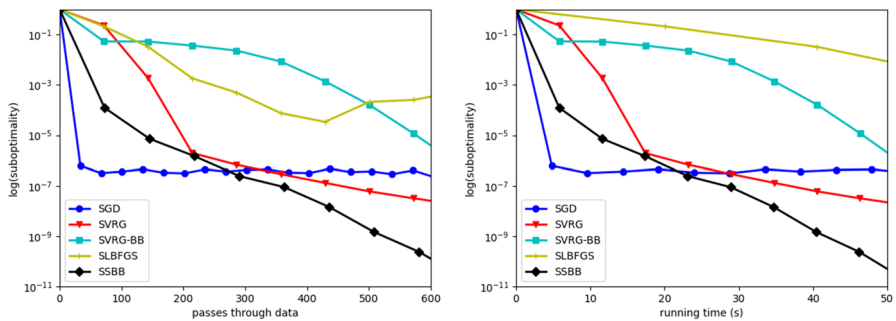
Fig. 3 l^2 -regularized squared hinge loss on a6a from LIBSVM regularized with \lambda_2 = 10^{-3} . Left : number of passes through data. Right : running time
