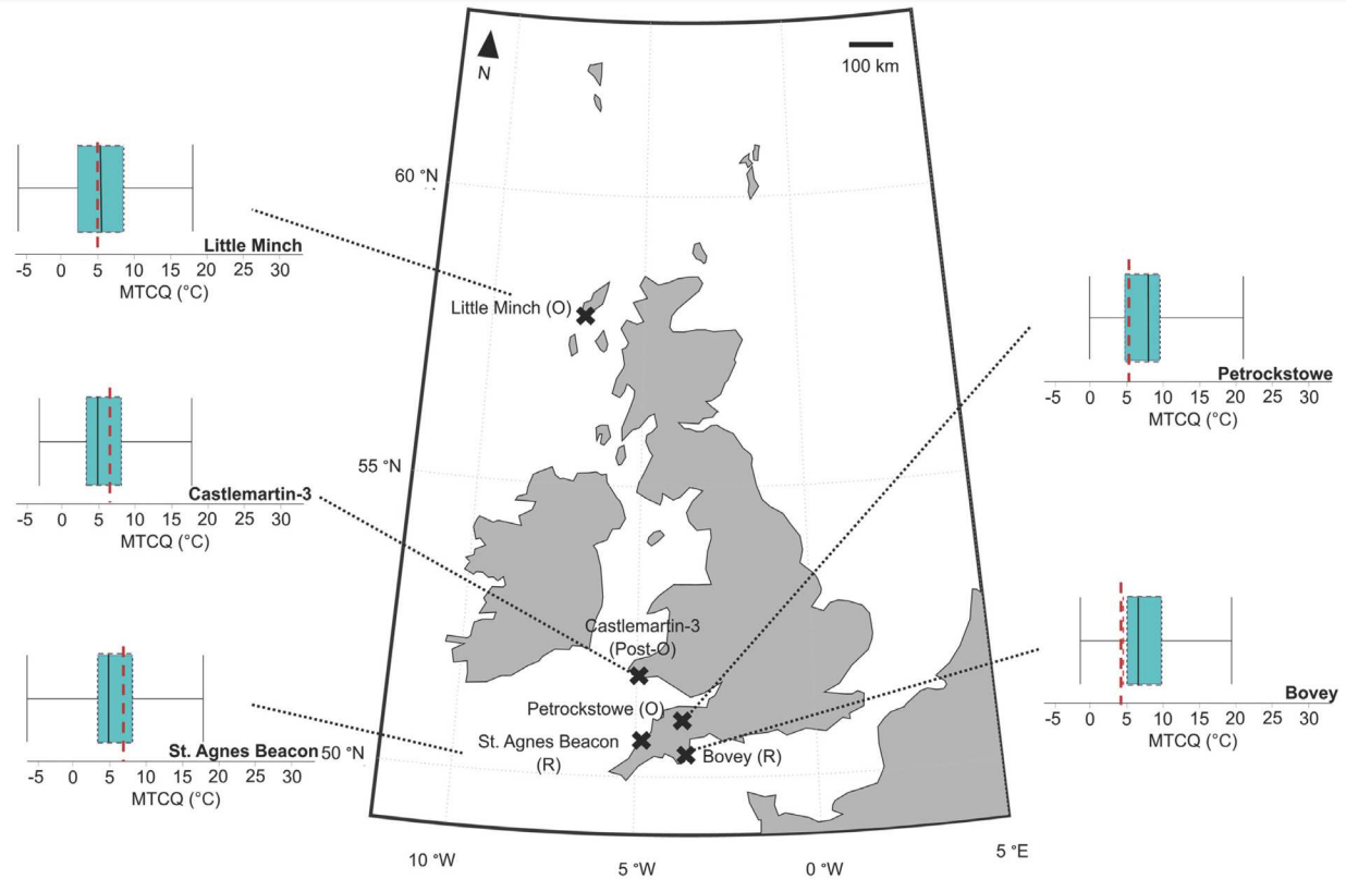
FIGURE 8. Mean Temperature of the Coldest Quarter (MTCQ) reconstructions, based on study sites where only one pollen assemblage was available. The red dotted line shows the present-day MTCQ. Solid black lines show the value of the reconstructed optima. The grey dotted lines and grey solid lines show the respective uncertainty ranges of 50 % and 95 %. Rupelian and Oligocene and ?Miocene sites are labelled (R) and (O), respectively.
