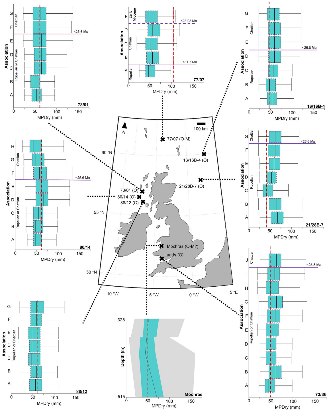
FIGURE 13. Mean Precipitation of the Driest Month (MPDry) reconstructions from the sequential boreholes. The red dotted line shows the present-day MPDry. Solid black lines show the value of the reconstructed optima. The grey dotted lines and grey solid lines show the respective uncertainty ranges of 50 % and 95 %. Oligocene and ?Miocene sites are labelled (O) and (M?), respectively. Purple solid lines and purple dotted lines separate Rupelian from Chattian, and Chattian from early Miocene associations, respectively, based on dinoflagellate cyst zonation. The uppermost/ lowermost ages of depicted boundaries between epochs, based on dinoflagellate cyst zonation, have been labelled where possible.
