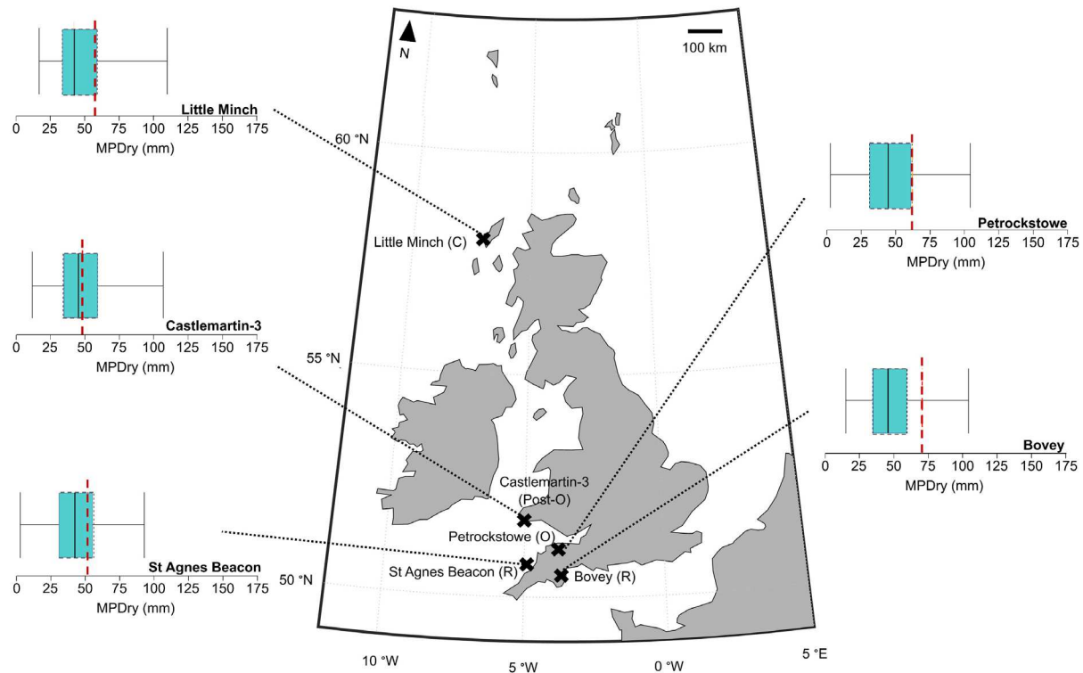
FIGURE 14. Mean Precipitation of the Driest Month (MPDry) reconstructions, based on study sites where only one pollen assemblage was available. The red dotted line shows the present-day MPRy. Solid black lines show the value of the reconstructed optima. The grey dotted lines and grey solid lines show the respective uncertainty ranges of 50 % and 95 %. Rupelian, Chattian and Oligocene sites are labelled (R), (C), and (O), respectively. Purple solid lines and purple dotted lines separate Rupelian from Chattian, and Chattian from early Miocene associations, respectively, based on dinoflagellate cyst zonation. The uppermost/ lowermost ages of depicted boundaries between epochs, based on dinoflagellate cyst zonation, have been labelled where possible.
