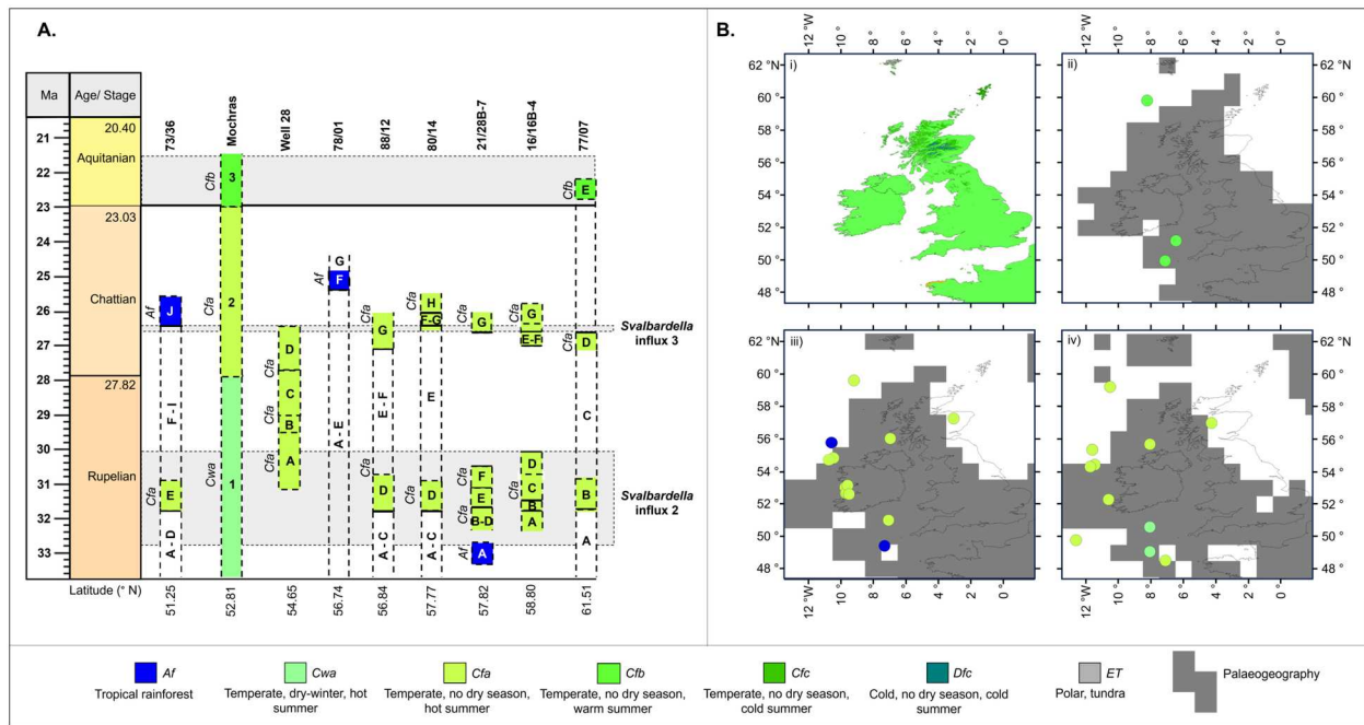
FIGURE 16. A. Köppen-Geiger signatures assigned to reconstructions of associations from Wilson (1996), and their likely age. The Mochras Basal Red Unit, the Transitional Unit and Lignite and Clay Units are labelled as 1-3, respectively. Age range of cooling Svalbardella -events 2 and 3, and their temporal overlaps with associations are labelled. Associations from Wilson (1996) are labelled alphabetically in accordance with original association assignment. Solid black lines in columns show a definitive age, based on dinoflagellate cyst stratigraphic age ranges. Dotted black lines in columns demonstrate an uncertain age range, based on dinoflagellate cysts stratigraphy. Dotted grey lines indicate possibility of age range regarding cooling events, i.e., Svalbardella -2, 3 and the early Miocene cooling. Latitude of boreholes are listed. B. Köppen-Geiger-based climate-type distributions across the British Isles, with key describing assigned climate types. Grey pixels show palaeogeography of British Isles (Scotese and Wright, 2018). Four stages are shown: i) Present-day Köppen-Geiger distribution of the British Isles (Beck et al., 2018); ii) Early Miocene; iii) Chattian; and iv) Rupelian.
