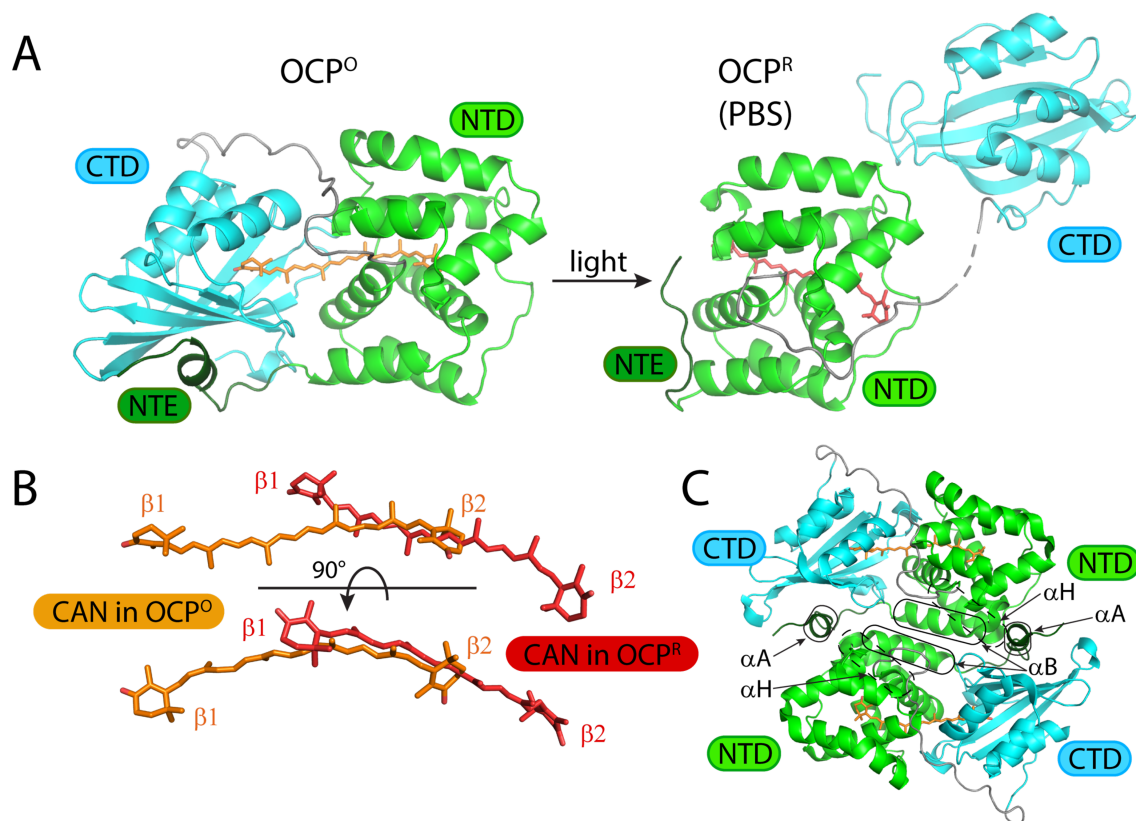
Figure 1. Structures of OCP 0 , OCP R , and the OCP 0 dimer. (a) Structures of the OCP 0 (left, pdb id 4xb5) with canthaxanthin (CAN, orange) and the phycobilisome (PBS)-bound form of OCP R (right, from the OCP-PBS structure, pdb id 7sc9) with CAN (red). C-terminal domains (CTD) are cyan, N-terminal domains (NTD) green, the N-terminal extension (NTE) dark green, and the connecting linkers grey. (b) Detailed view showing the translocation of CAN in OCP 0 (orange) and OCP R (red) in two orientations, indicating the \beta -ionone rings in the CTD and NTD, \beta_1 and \beta_2 , respectively. (c) Overview of the OCP 0 dimer as observed in the crystal structure of Synechocystis sp. PCC 6803 OCP (pdb id 4xb5), with the \alpha helices labeled that form the major interaction surface between the two monomers.
