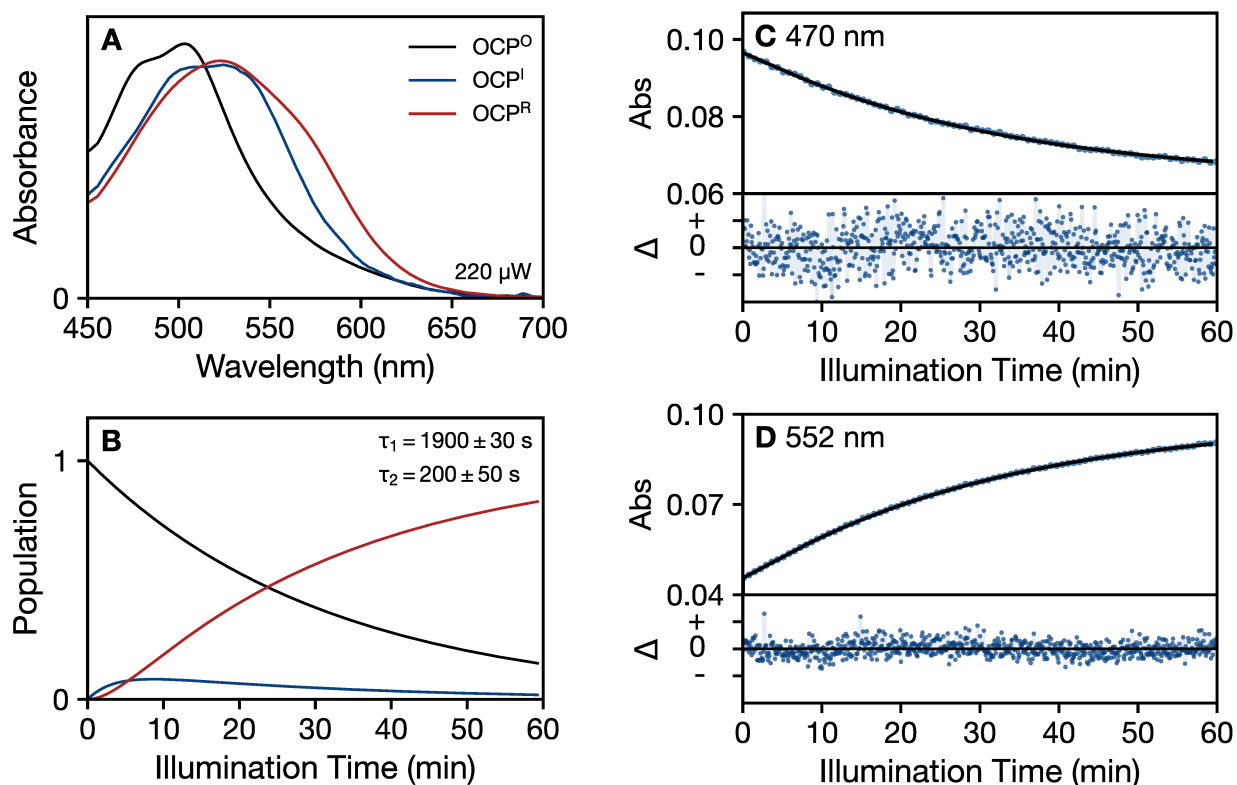
Figure 3. Global modeling of the time evolution of the absorption spectrum of OCP at 273 K in the presence of 60% (v/v) glycerol under continuous 430-nm illumination (220 \mu W), applying a three-compartment kinetic model: OCP^0 \xrightarrow{1/\tau_1} OCP^I \xrightarrow{1/\tau_2} OCP^R . (a) Evolution-associated absorption spectra for the three kinetic compartments: dark-adapted OCP^0 reactant (black), the OCP^I intermediate (blue), and the final OCP^R product (red). (b) Time evolution of the populations for the OCP^0 , OCP^I , and OCP^R kinetic compartments. (c, d) Fit of the global model (black) to the observed absorption (blue dots) at two detection wavelengths, 470 nm and 552 nm, as marked in Fig. 2a and b, showing the single-wavelength absorption transients (top panel) and residuals (bottom panel). The residuals ( \Delta = data – global model) are shown with a 20 \times zoom factor for the absorbance ordinate.
