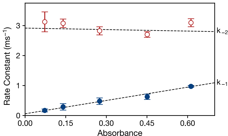
Figure 7. Concentration dependence of the first-order rate constants determined by global modeling of the dark recovery of OCP at 293 K in the absence of glycerol following illumination at 430 nm. The absorption ( A ) of the dark adapted OCP 0 sample was measured at 500 nm prior to exposing the sample to light. Supplemental Figs. S16 and S17 show the global models for the dark recovery measured for the OCP samples with absorbances of 0.06 and 0.6. The dashed lines show fitted linear models: k_{-1} = (1.48 \pm 0.10) \times A + (0.060 \pm 0.050) \text{ ms}^{-1} , and k_{-2} = (-0.17 \pm 0.36) \times A + (2.95 \pm 0.15) \text{ ms}^{-1} .
