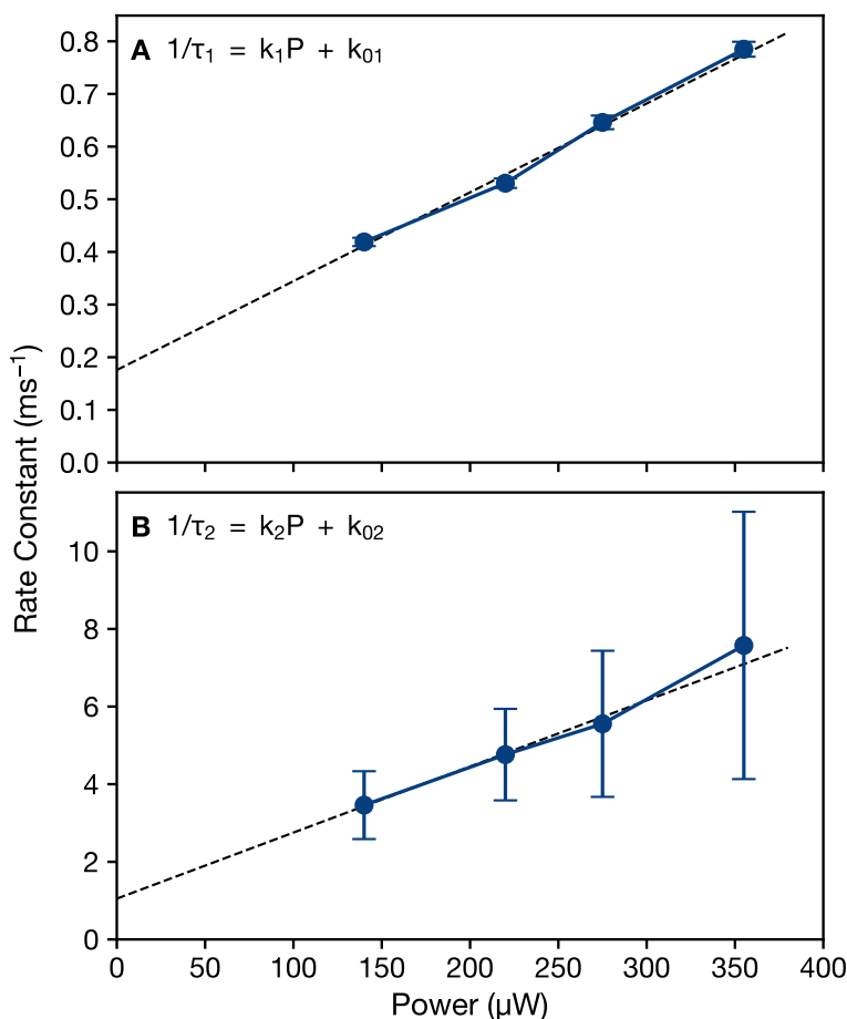
Figure 4. Dependence of the photoactivation rate constants observed at 273 K in the presence of 60% (v/v) glycerol on the incident total power of the 430-nm excitation beam for (a) \text{OCP}^0 \xrightarrow{1/\tau_1} \text{OCP}^I and (b) \text{OCP}^I \xrightarrow{1/\tau_2} \text{OCP}^R , as determined by two-step global models. The error bars show the 95% confidence limits for the measured rates at a given illumination power. The dashed lines are least-squares fits to the linear model 1/\tau = kP + k_0 , where k is the rate constant, P is the illumination power, and k_0 is the rate due to the white-light
