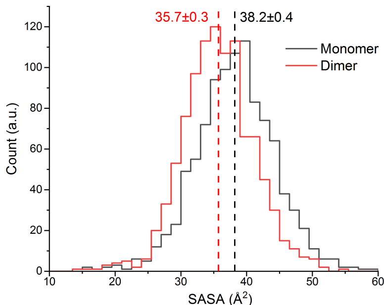
Figure 9. Distribution of the solvent accessible surface area (SASA) for the canthaxanthin chromophore in the OCP 0 monomer (black) and dimer (red) structures from molecular dynamics (MD) trajectories at 300 K. The dotted vertical lines mark the average values, which are labeled with 95% confidence intervals due to the standard deviation of the mean for the 1000 samples in the MD trajectory. The distributions are characterized by the standard deviations 5.4 Å 2 for the dimer and 6.0 Å 2 for the monomer. See the Supplementary Information for details about the MD simulations used to calculate the SASA.
