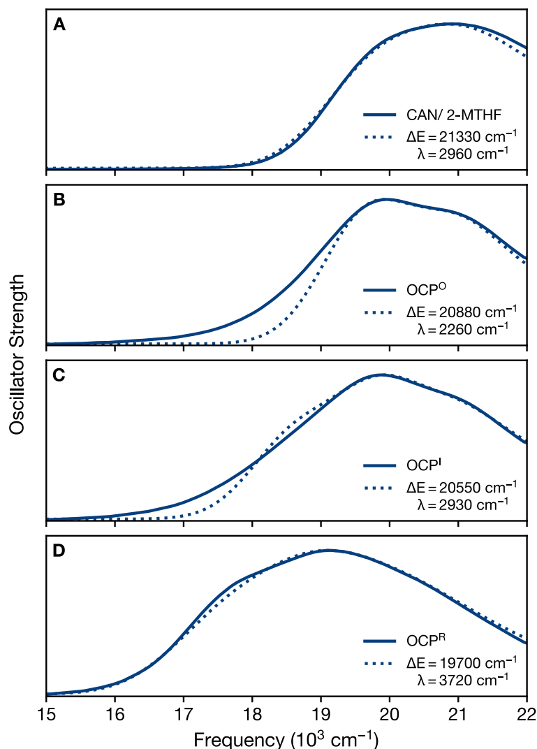
Figure 8. Numerical simulations (dotted spectra) using the multimode Brownian oscillator (MBO) model of the experimental absorption oscillator strength spectra (solid spectra) for (a) canthaxanthin (CAN) in 2-methyltetrahydrofuran solvent and (b–d) of the evolution-associated spectra for three components in the photoactivation global model at 293 K in the absence of glycerol (from Fig. 6). The absorption spectra are plotted here as the oscillator strength, \varepsilon(\nu)^3/\nu , where \varepsilon gives the absorbance and \nu stands for the frequency. The MBO model parameters for each of the simulated spectra are listed in the Supplementary Information in Table S1. The legends for panels (a–d) give the values for the vertical ground-to-excited-state energy gap, \Delta E , and the reorganization energy, \lambda , in wavenumbers ( \text{cm}^{-1} ).
