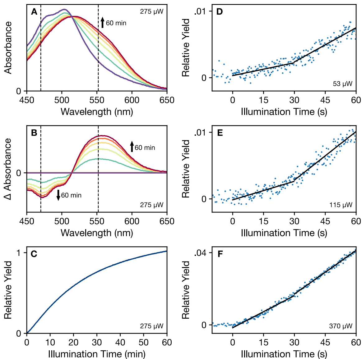
Figure 2. Photoactivation assays of dark-adapted OCP at 273 K in the presence of 60% (v/v) glycerol under continuous 430-nm illumination (275 \mu W). (a) Time evolution of the absorption spectrum from zero illumination (purple) to 60 min of illumination (dark red), with intermediate spectra spaced by 12 min of illumination. (b) Difference absorption spectra (light – dark adapted) for the set of spectra shown in panel (a). The vertical dashed lines shown in (a, b) mark the wavelengths used for the transients in Fig. 3. (c) Time course of the relative yield of the OCP R product, determined from the integral of the absolute value of the difference spectrum. (d–f) Time courses of the relative yields of OCP R at short illumination times with increasing illumination power: 53 \mu W, 115 \mu W, and 370 \mu W,
