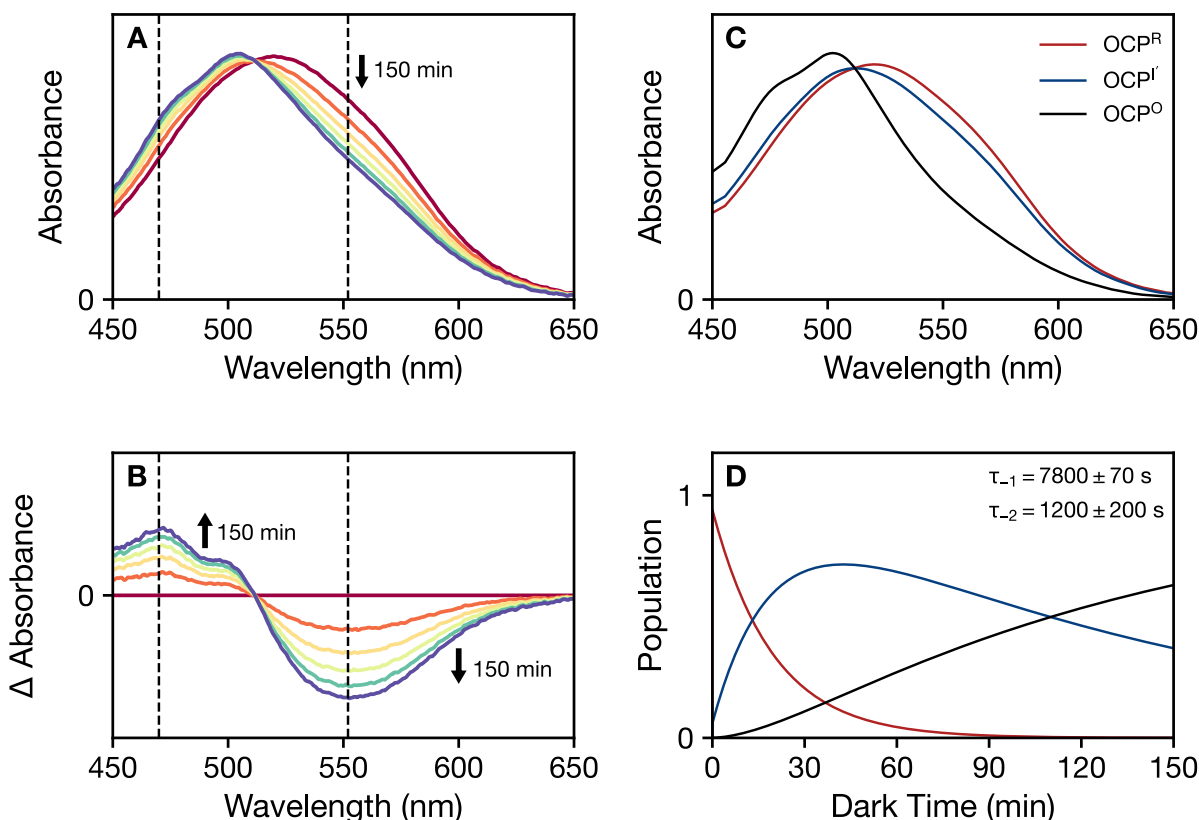
Figure 5. Dark recovery of photoactivated OCP at 293 K in the presence of 60% (v/v) glycerol following continuous 430-nm illumination (275 \mu W) for 30 min. (a) Time evolution of the absorption spectrum from zero dark time (red) to 150 min of darkness (purple), with intermediate spectra spaced by 30 min of darkness. (b) Difference absorption spectra (increasing dark time – initial spectrum after illumination) for the set of spectra shown in panel (a). (c, d) Evolution-associated spectra and populations for a two-step kinetic model: \text{OCP}^{\text{R}} \xrightarrow{1/\tau_2} \text{OCP}^{\text{I}} \xrightarrow{1/\tau_1} \text{OCP}^{\text{O}} . Supplementary Figs. S5 and S6, respectively, show the fitted transients and residuals for the one-step and two-step global models, respectively. Panel (d) indicates the initial populations (boundary conditions) for the dark recovery, which were determined from a global model for the forward, photoactivation response: \text{OCP}^{\text{R}}(0) = 0.94 , \text{OCP}^{\text{I}}(0) = 0.06 , and \text{OCP}^{\text{O}}(0) = 0.00 . The rates and the associated
