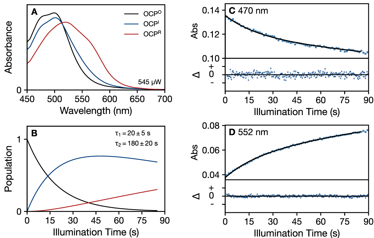
Figure 6. Global modeling of the time evolution of the absorption spectrum of OCP at 293 K in the absence of glycerol under continuous 430-nm illumination (545 \mu W), applying a three-compartment kinetic model: \text{OCP}^0 \xrightarrow{1/\tau_1} \text{OCP}^I \xrightarrow{1/\tau_2} \text{OCP}^R . (a) Evolution-associated absorption spectra for the three kinetic compartments: dark-adapted \text{OCP}^0 reactant (black), the \text{OCP}^I intermediate (blue), and the final \text{OCP}^R product (red). (b) Time evolution of the populations for the \text{OCP}^0 , \text{OCP}^I , and \text{OCP}^R kinetic compartments. (c, d) Fits of the global model (black) to the observed absorption (blue dots) at two detection wavelengths, 470 nm and 552 nm, showing the single-wavelength absorption transients (top panel) and residuals (bottom panel). The residuals ( \Delta = \text{data} - \text{global model} ) are shown with a 20 \times zoom factor for the absorbance ordinate.
