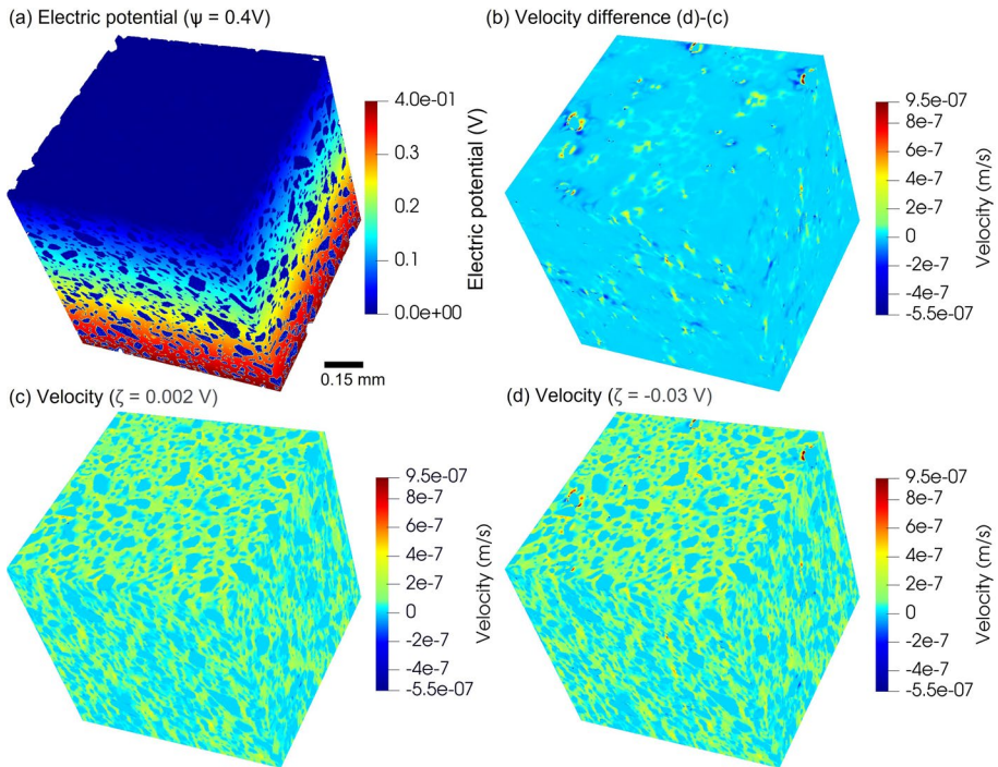
Fig. 4 Simulation results for Domain1: a electric potential; b fluid velocity difference between chalcopyrite \zeta of 0.002 V and -0.03 V; c fluid velocity profile of \zeta = 0.002 V; d fluid velocity profile of \zeta = -0.03 V
