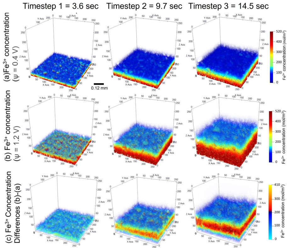
Fig. 7 \text{Fe}^{3+} distribution in Domain1 under different external \psi : a \psi = 0.4 \text{ V} ; b \psi = 1.2 \text{ V} . c Differences in \text{Fe}^{3+} distributions between (a) and (b)
