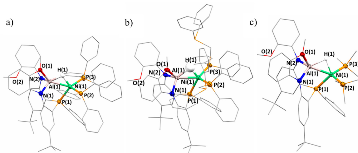
Fig. 2 Solid-state structures of (a) 2-(PPh 3 ) 2 , (b) 2-(dppe) 2 , and (c) 2-(PMe 3 ) 2 . Hydrogen atoms on ligands are excluded for clarity. Mixed wire-frame/ellipsoid view used for clarity.
