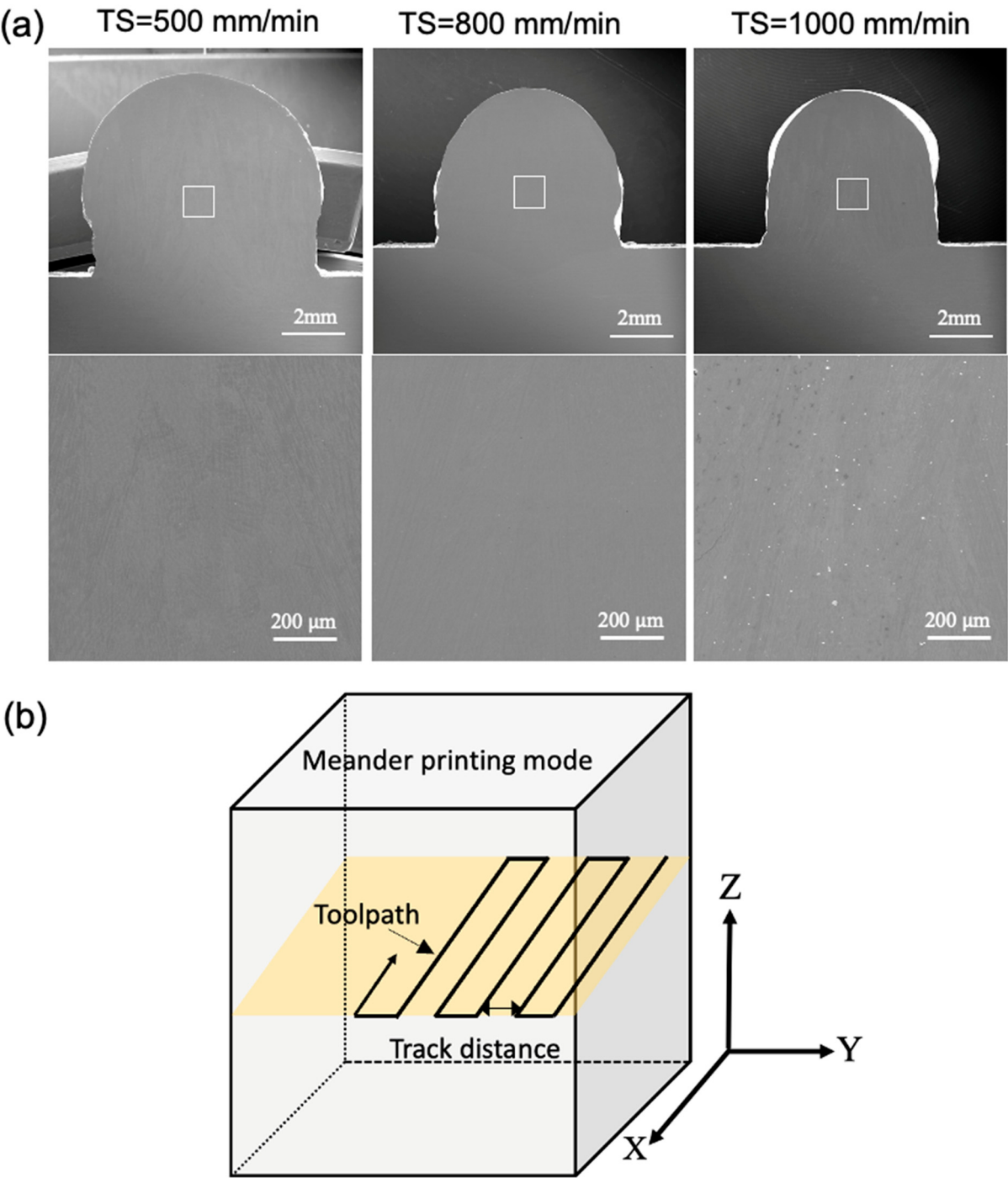
Figure 1. (a) SEM image (based on secondary electron diffraction) of (upper panel) cross-section of the single-bead 3-layer build and (lower panel) magnified SEM image of selected area in the upper panel
