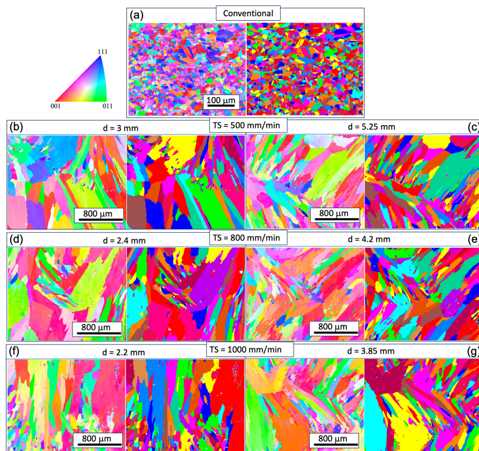
Figure 4. IPF maps for grain orientation and grain structure maps on the YZ plane at different track distances (d) with respective torch speed (TS) as follows: TS = 500 mm/min, 800 mm/min, and 1000 mm/min; subfigure (a) corresponds to the conventional sample, and subfigures (b–g) correspond to WAAM samples 1–6.
