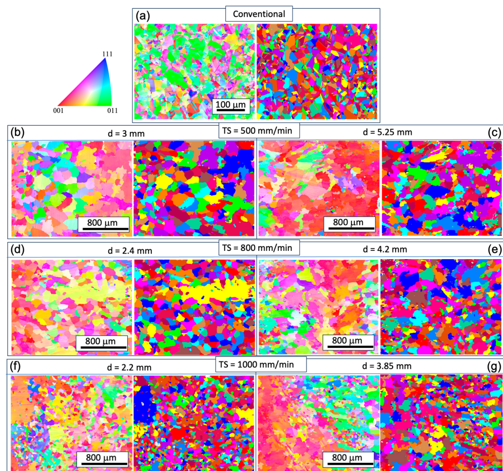
Figure 3. IPF maps for grain orientation and grain structure maps on the XY plane at different track distances ( d ) with respective torch speed (TS) as follows: TS = 500 mm/min, 800 mm/min, and 1000 mm/min; subfigure (a) corresponds to the conventional sample, and subfigures (b–g) correspond to WAAM samples 1–6.
