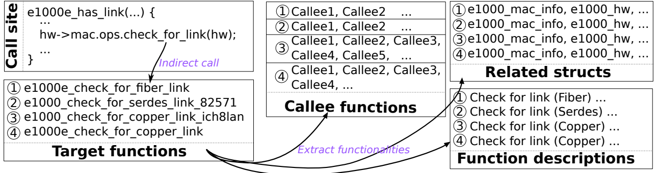
Fig. 3: Abstractive information of target functions. Callee1 to Callee5 are e1000e_config_fc_after_link_up , e_dbg , e1000e_phy_has_link_generic , e1000e_check_downshift , and e1000e_get_speed_and_duplex_copper .
