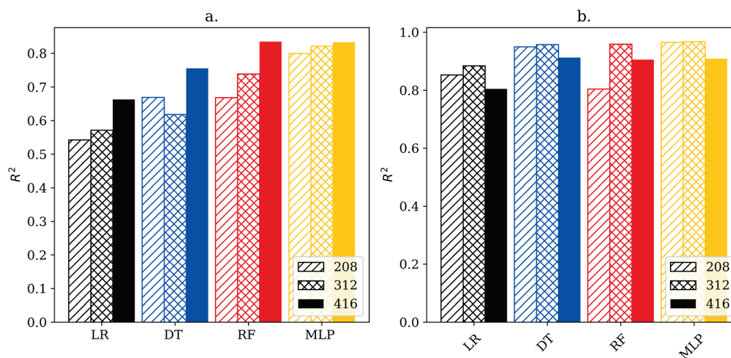
Fig. 2 Coefficient of determination ( R^2 ) of decision tree (DT), random forest (RF), multilayer perceptron (MLP) and linear regression (LR) predicting both faradaic efficiency (a) and NRR rate (b) over various data set sizes.
