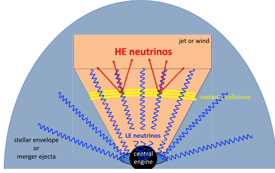
FIG. 1. Schematic picture of \text{HE}\nu (GeV–PeV) production and their interactions with \text{LE}\nu s (MeV–GeV) from the central engine such as a black hole with an accretion disk or a newborn magnetar. \text{HE}\nu production occurs at R_{\text{diss}} \gg R_{\text{eng}} , which may be beamed with the opening angle \sim 1/\Gamma , with R_{\text{diss}} , R_{\text{eng}} , and \Gamma being the dissipation radius, engine radius, and outflow Lorentz factor, respectively. Note that the opening angle of the \text{LE}\nu beams is exaggerated for illustration purposes.
