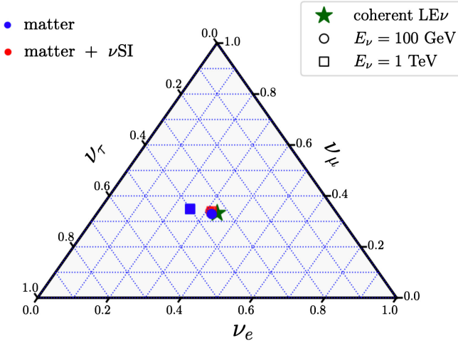
FIG. 3. Expected \nu_e:\nu_\mu:\nu_\tau ratio on Earth in the absence and presence of \nu SI for different neutrino energies. Note that the matter effect is included in both cases, assuming the density profile of a blue supergiant, and the ratio with \nu SI is very close to the total flavor equipartition. In addition, the green star indicates the total flavor equipartition expected from the propagation of HE \nu s in a bath of oscillating LE \nu s, as discussed in the text. Note that, apart from the matter-only case for the 1 TeV neutrinos, the other ones are almost on top of each other. It is also illuminating to keep in mind that the final flavor states are specific to the initial flavor composition of 1:2:0 and can vary under different circumstances.
