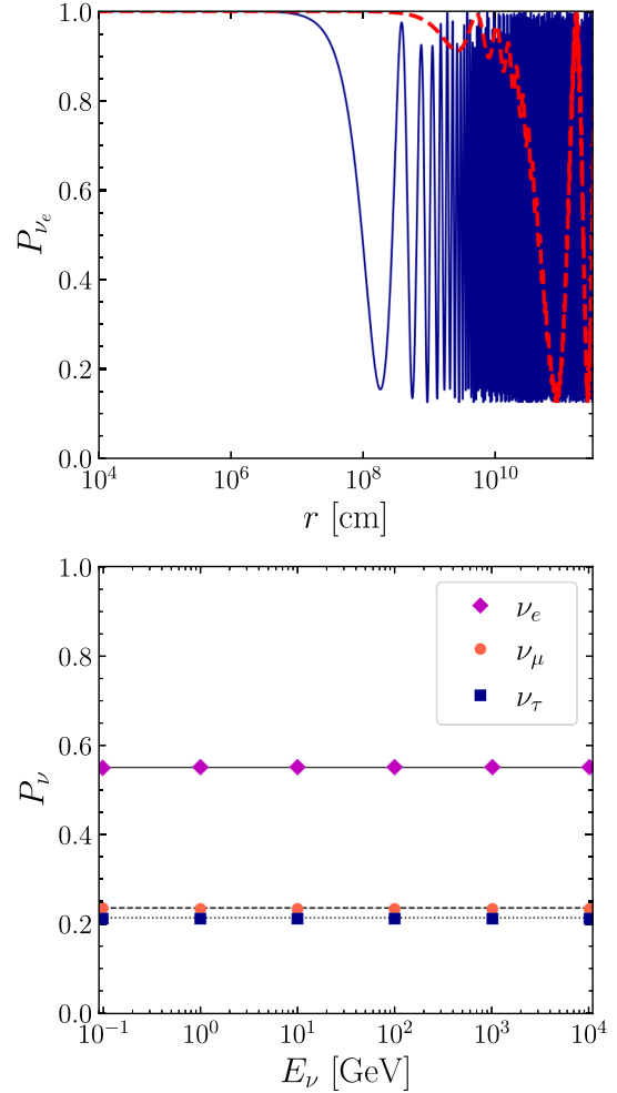
FIG. 2. Top: survival probability of \text{HE}\nu_e 's propagating in vacuum (dashed red curve), and in the bath of the \text{LE}\nu s (solid blue curve). \text{HE}\nu s can experience flavor conversions on scales much shorter than those expected in vacuum. Here, for illustrative purposes, we assume \mu = 10^{-7} \text{ cm}^{-1} , E_{\text{LE}\nu} = 10 \text{ MeV} , and E_{\text{HE}\nu} = 100 \text{ GeV} . For the \text{LE}\nu bath, n_{\bar{\nu}_e}/n_{\nu_e} = 1.3 is also fixed, although the survival probabilities are independent of n_{\bar{\nu}_e}/n_{\nu_e} as long as it is not too close to 1. Bottom: survival probabilities as a function of the \text{HE}\nu energy, where the diamonds, points, and squares are the survival probabilities of \nu_e , \nu_\mu , and \nu_\tau obtained from the simulations, respectively, and the black lines are the corresponding analytical solutions. We assume an initial flavor ratio of \nu_e:\nu_\mu:\nu_\tau = 1:0:0 . Here we set \theta_{12} = 33.6^\circ , \theta_{23} = 47.2^\circ , \theta_{13} = 8.5^\circ , and \delta_{\text{CP}} = 0 . Antineutrinos behave in exactly the same manner.
