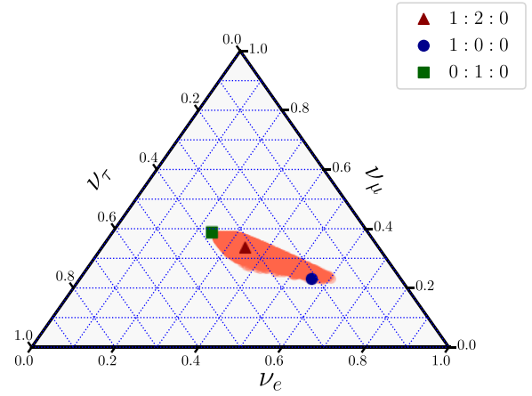
FIG. 4. Expected \nu_e:\nu_\mu:\nu_\tau ratio after HE \nu s escape their production region, in the presence of \nu NSSI. The triangle, circle, and square indicate the ratio in the SM while the red region shows how the ratio changes in the presence of \nu NSSI for the 1:2:0 case. Here the red region is created by choosing a large set of randomly populated \hat{G}^{\alpha\beta} assuming that |\hat{G}^{\alpha\beta}| < 1 (for \alpha \neq \beta ). Via coherent \nu SI, the final HE \nu flavor ratio is very sensitive to the \nu NSSI.
