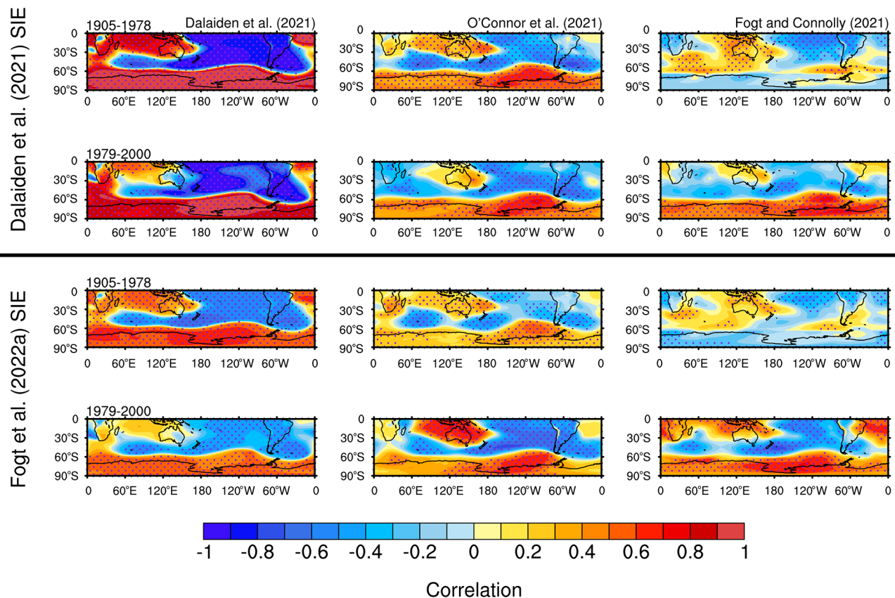
Figure 7. Annual mean correlations of (top half) Dalaide et al. (2021a) and (bottom half) Fogt et al. (2022a) sea ice extent correlations for the Weddell Sea with three 20th century spatially complete pressure reconstructions (columns). In each half, the top row represents correlations in the pre-satellite period of 1905–1978, and the bottom row is for 1979–2000. The pressure reconstructions are from (left column panels) Dalaide et al. (2021a), (middle column panels) O'Connor et al. (2021a), and (right column panels) Fogt and Connolly (2021). Correlations statistically different from zero at p < 0.05 are stippled.
