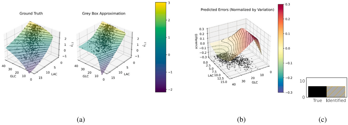
Fig. 14. Comparison of fluxes (stoichiometric ground-truth vs. gray-box model). 14(a): ground-truth and neural net approximations of the fluxes as functions of the learned kinetic expression inputs GLC and LAC 14(b): normalized (as in Figs. 11(b) and 12(b)) predicted errors Black data points plotted as in Figs. 11 and 12. 14(c): Ground-truth value and the recovered value of the kinetic parameter \alpha_1 .
