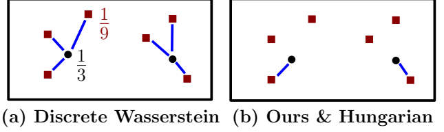
Figure 3: Distance between prediction (red) and GT (black). Discrete Wasserstein gives a fractal mass to each point and matches all of them (blue lines). Our method only conducts one-to-one matching. Unmatched points get a large penalty. Hungarian loss drops unmatched points.
