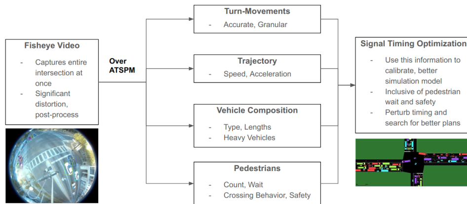
Figure 3: Flowchart showing the workflow for using fisheye video data to improve safety and signal timing of an intersection using a traffic microsimulation framework. Fisheye video data provides vital information on different aspects of the intersection dynamics, which can then be used to improve modeling.
