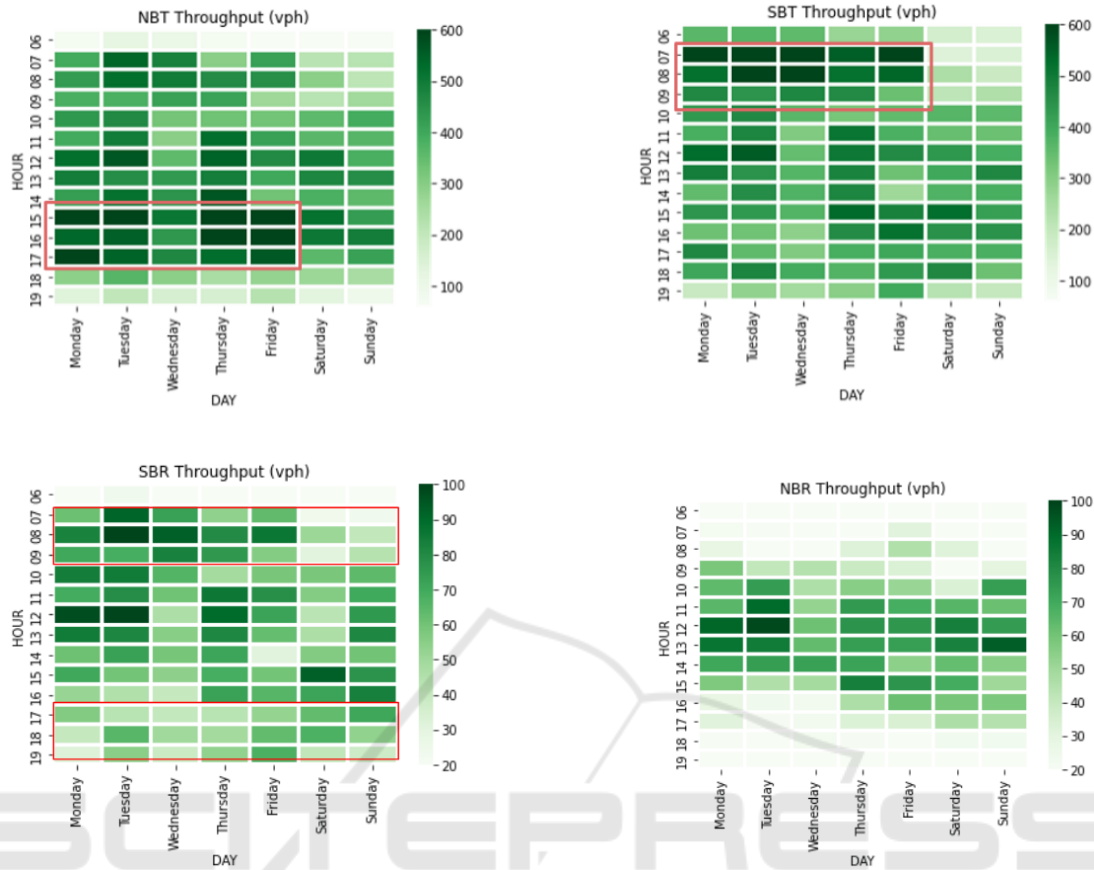
Figure 4: Heatmap showing the intensity of vehicles per hour for various hours of the day across the week. We can see that the Southbound-through direction has a larger AM peak, and the Northbound-through direction sees a larger PM peak. This is likely because the University is south of the intersection, with people coming to work in the morning and leaving in the evening. Similarly, for Southbound-Right and Northbound-Right directions, we can see that both AM and PM peaks for Southbound-Right are larger. Loop detectors do not usually capture right turns as they share the same lane as through movements. Right turns are vital for pedestrian safety, as drivers may neglect pedestrians while focusing on merging at the right turn.
