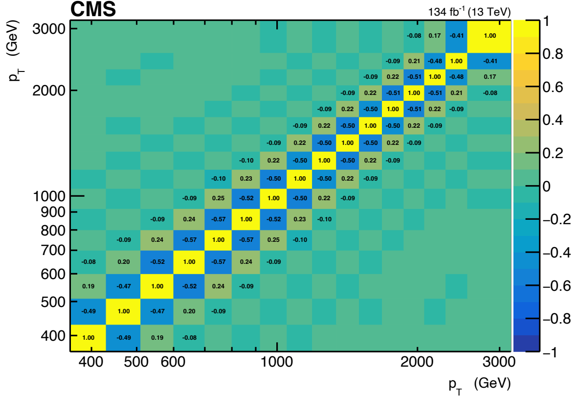
Figure 3: Bin-to-bin correlation matrix for the R_{\Delta\phi}(p_T) distribution at the particle level, where the value 1 (−1) corresponds to fully (anti)correlated bins. For illustration purposes, only bins with (anti)correlations larger (smaller) than 0.05 (−0.05) are shown also as text.
