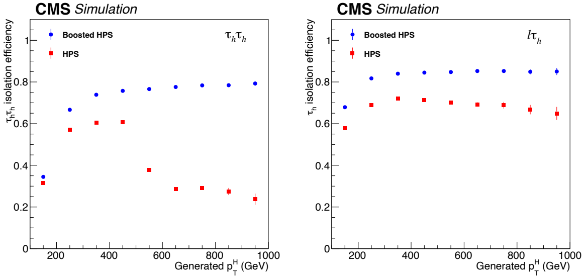
Figure 1: Comparison of the isolation efficiencies for the standard and boosted HPS algorithms in the \tau_h\tau_h (left) and \ell\tau_h (right) final states.
