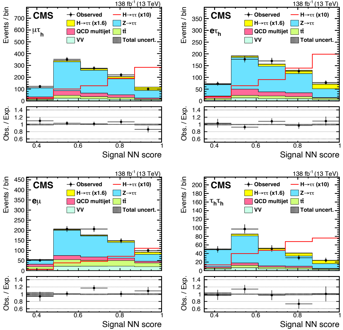
Figure 2: Observed and expected NN distributions in the SR, after combining all four p_T^H bins, in the \mu\tau_h (upper left), e\tau_h (upper right), e\mu (lower left), and \tau_h\tau_h (lower right) channels. The signal and background distributions are the result of a simultaneous binned maximum likelihood fit to all three output NN distributions, including all individual p_T bins and data-taking years. The bottom panel shows the ratio of the number of events observed in data to that of the expected background.
