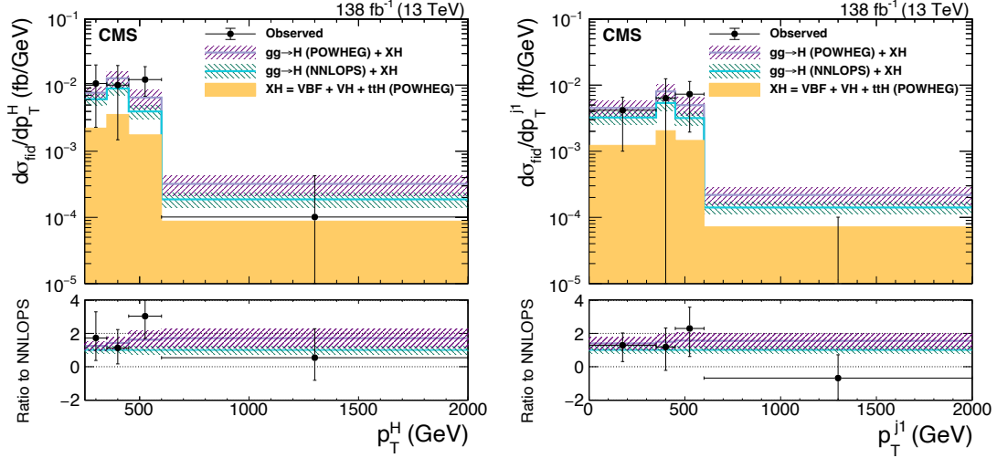
Figure 3: Observed and expected differential fiducial cross sections in bins of p_T^H (left) and p_T^{j1} (right). The last bins include the overflow. The uncertainty bands in the theoretical predictions include uncertainties from the following sources: PDF, renormalization and factorization scales, underlying event and parton showering, and the branching fraction \mathcal{B}(H \rightarrow \tau\tau) .
