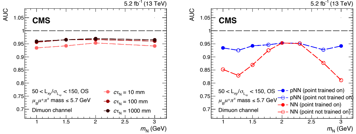
Figure 4: (Left) Performance of the pNN as a function of signal mass for events in the 50 < L_{xy}/\sigma_{L_{xy}} < 150 , OS, and low \ell_B \ell^\pm \pi^\mp mass category in the dimuon channel. The performance is shown by the AUC curve, where a value at unity corresponds to a perfect separation between signal and background. The different coloured curves correspond to different c\tau_N hypotheses. (Right) Validation of the use of a pNN for intermediate m_N mass points, for events in the 50 < L_{xy}/\sigma_{L_{xy}} < 150 , OS and low \ell_B \ell^\pm \pi^\mp mass category in the dimuon channel: a pNN trained on masses m_N = 1.0, 1.5, 2.0 , and 3.0 GeV (blue) and a NN trained on mass m_N = 2 GeV (red). All the points have c\tau_N = 10 mm. The full circles correspond to mass points on which the pNN and NN were trained on, while the open circles show mass points that have not been trained on.
