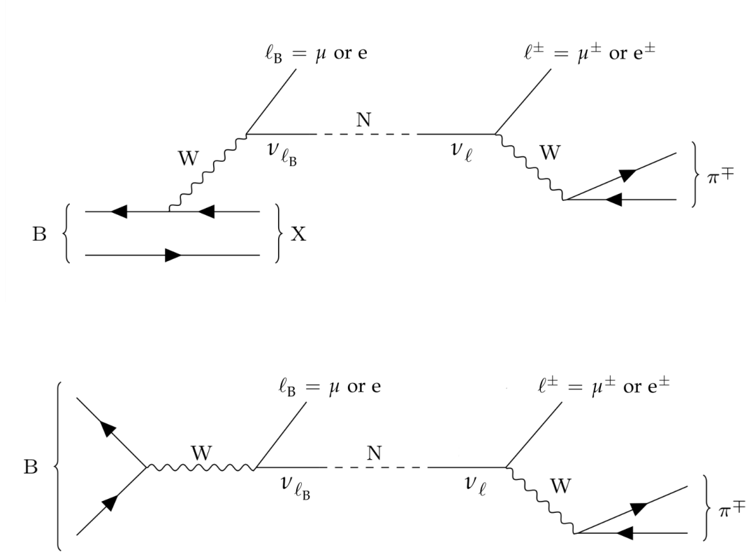
Figure 1: Feynman diagrams showing the semileptonic (upper row) and leptonic (lower row) decay of a B meson into a lepton ( \ell_B ), a hadronic system (X) in case of the semileptonic decay, and a neutrino ( \nu_{\ell_B} ), which contains a small admixture of a heavy neutrino (N). The N mass eigenstate propagates and, according to its admixture of the neutrino flavour eigenstate ( \nu_\ell ), decays weakly into a lepton \ell^\pm and a charged pion \pi^\mp .
