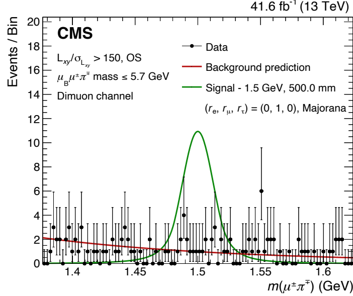
Figure 7: Distribution of the \mu^\pm \pi^\mp invariant mass in the mass window around 1.5 GeV in the high L_{xy}/\sigma_{L_{xy}} , OS, and low \ell_B \ell^\pm \pi^\mp mass category in the dimuon channel. The result of the background-only fit to the data (red) is shown together with the mass distribution expected from a Majorana signal with m_N = 1.5 GeV and c\tau_N = 500 mm, for the case in which the N mixes with the muon sector only (green).
