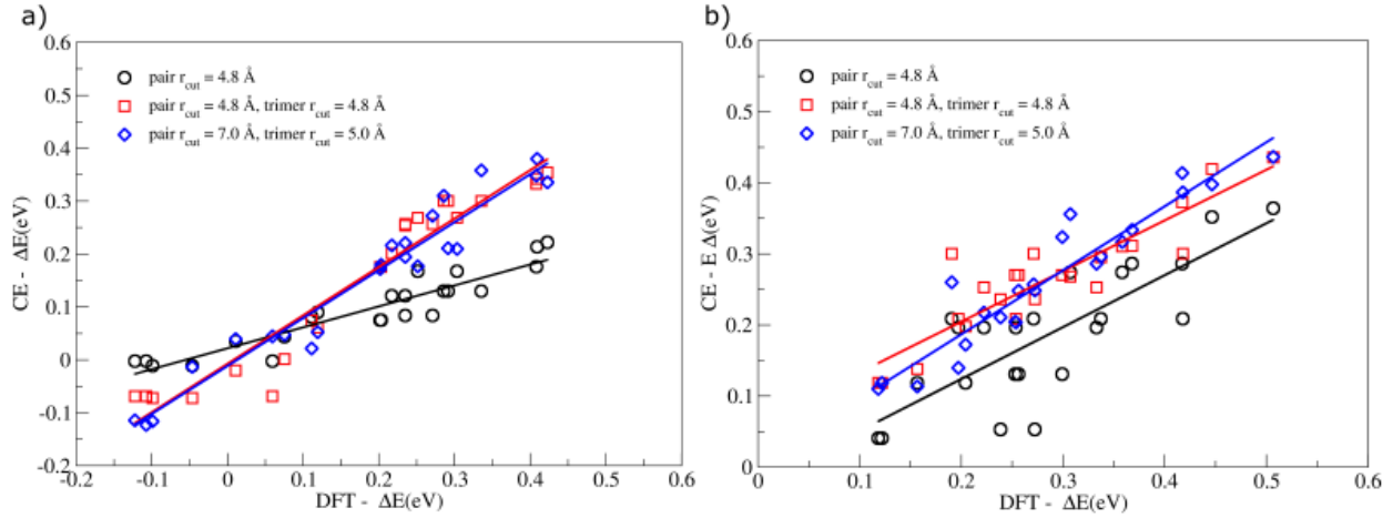
Figure 7: Parity plot of adsorption energies obtained by CE (LOOCV values) and DFT for a) *CO and b) *COOH adsorption on Cu 3 Au(111). The results from CE were obtained considering only pair or pair and trimer clusters with different values of cutoff radius, r_{\text{cut}} , for the clusters included in the expansion.
