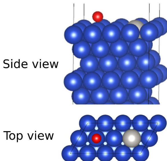
Figure 8: Representation of pair cluster with the largest contribution to the ^*\text{CO} and ^*\text{COOH} adsorption energies as predicted by the cluster expansion, apart from the clusters that contain the atom near the adsorbate and its first nearest neighbors. The red sphere represents the adsorbate binding site, while gray (blue) spheres represent atoms that are (are not) present in the cluster.
