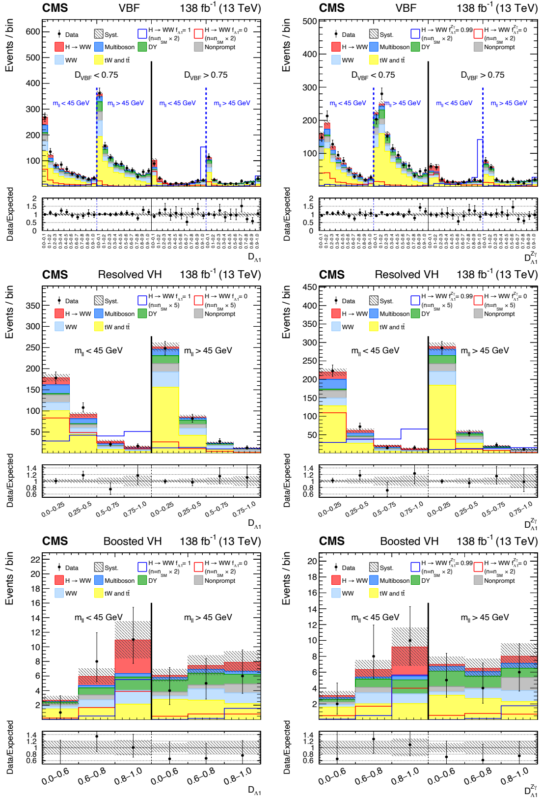
Figure 5: Observed and predicted distributions after fitting the data for [D_{VBF}, m_{\ell\ell}, D_{A1}] (upper left) and [D_{VBF}, m_{\ell\ell}, D_{A1}^{Z\gamma}] (upper right) in the VBF channel, and for [m_{\ell\ell}, D_{A1}] (left) and [m_{\ell\ell}, D_{A1}^{Z\gamma}] (right) in the Resolved VH (middle) and Boosted VH (lower) channels. For the fits, the a_1 and \kappa_1/(\Lambda_1)^2 (left) or a_1 and \kappa_2^{Z\gamma}/(\Lambda_1^{Z\gamma})^2 (right) HVV coupling contributions are included. More details are given in the caption of Fig. 3.
