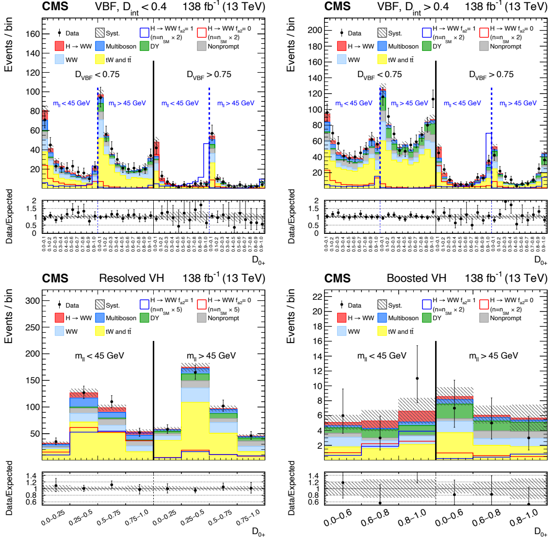
Figure 3: Observed and predicted distributions after fitting the data for [D_{\text{VBF}}, m_{\ell\ell}, D_{0+}] in the VBF channel (upper), and for [m_{\ell\ell}, D_{0+}] in the Resolved VH (lower left) and Boosted VH (lower right) channels. For the VBF channel, the D_{\text{int}} < 0.4 (left) and D_{\text{int}} > 0.4 (right) categories are shown. The predicted Higgs boson signal is shown stacked on top of the background distributions. For the fit, the a_1 and a_2 HVV coupling contributions are included. The corresponding pure a_1 ( f_{a_2} = 0 ) and a_2 ( f_{a_2} = 1 ) signal hypotheses are also shown superimposed, their yields correspond to the predicted number of SM signal events scaled by an arbitrary factor to improve visibility. The uncertainty band corresponds to the total systematic uncertainty. The lower panel in each figure shows the ratio of the number of events observed to the total prediction.
