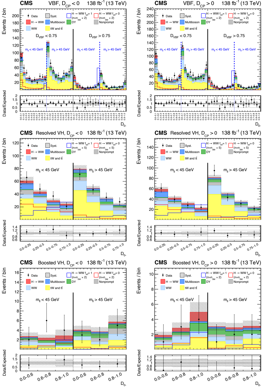
Figure 4: Observed and predicted distributions after fitting the data for [D_{VBF}, m_{\ell\ell}, D_0] in the VBF channel (upper), and for [m_{\ell\ell}, D_0] in the Resolved VH (middle) and Boosted VH (lower) channels. For each channel, the D_{CP} < 0 (left) and D_{CP} > 0 (right) categories are shown. For the fit, the a_1 and a_3 HVV coupling contributions are included. More details are given in the caption of Fig. 3.
