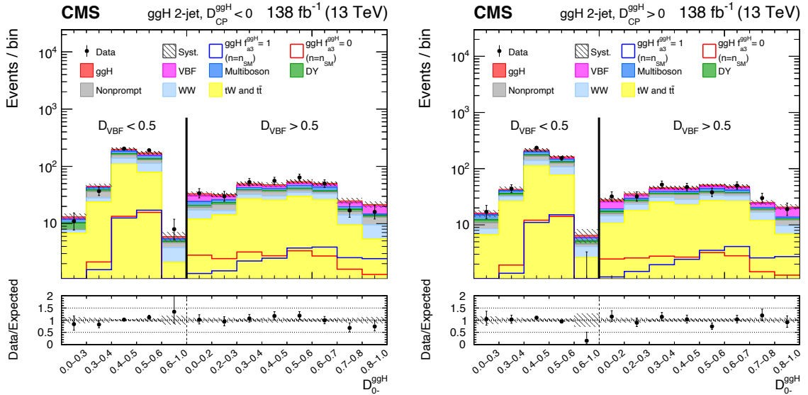
Figure 7: Observed and predicted distributions after fitting the data for [D_{\text{VBF}}, D_0^{\text{ggH}}] in the 2-jet ggH channel. Both the D_{\text{CP}}^{\text{ggH}} < 0 (left) and D_{\text{CP}}^{\text{ggH}} > 0 (right) categories are shown. In this case, the VBF and ggH signals are shown separately. For the fit, the a_2^{\text{gg}} and a_3^{\text{gg}} coupling contributions are included. The corresponding pure a_2^{\text{gg}} ( f_{a3}^{\text{ggH}} = 0 ) and a_3^{\text{gg}} ( f_{a3}^{\text{ggH}} = 1 ) signal hypotheses are also shown superimposed, their yields correspond to the predicted number of SM signal events. More details are given in the caption of Fig. 3.
