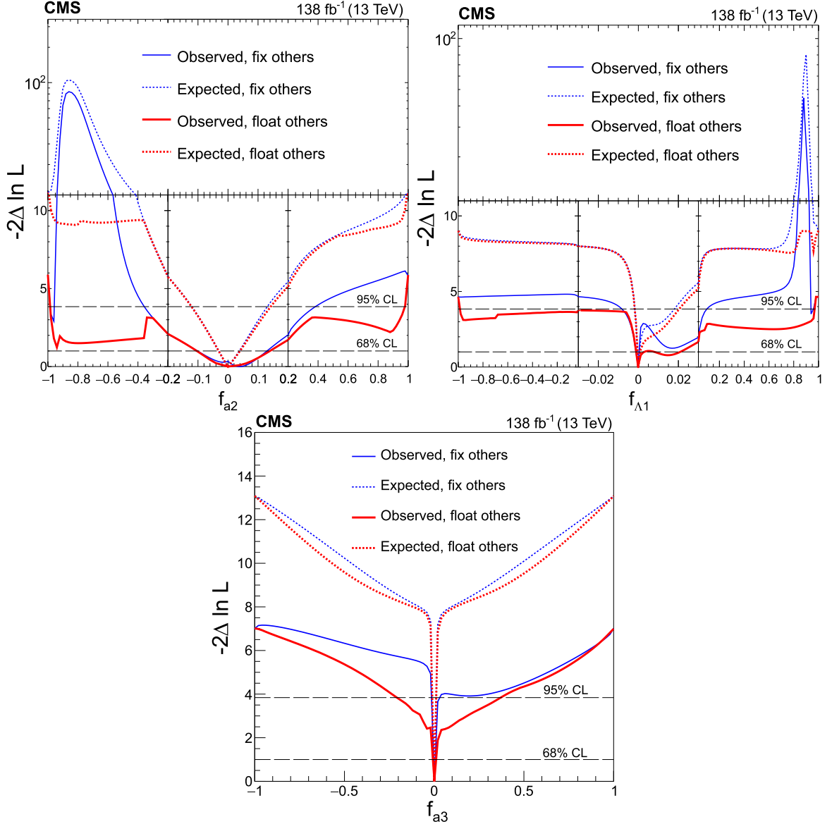
Figure 9: Expected (dashed) and observed (solid) profiled likelihood on f_{a2} (upper left), f_{\Lambda1} (upper right) and f_{a3} (bottom) using Approach 2. The other two anomalous coupling cross section fractions are either fixed to zero (blue) or left floating in the fit (red). In each case, the signal strength modifiers are treated as free parameters. The dashed horizontal lines show the 68 and 95% CL regions. Axis scales are varied for f_{a2} and f_{\Lambda1} to improve the visibility of important features.
