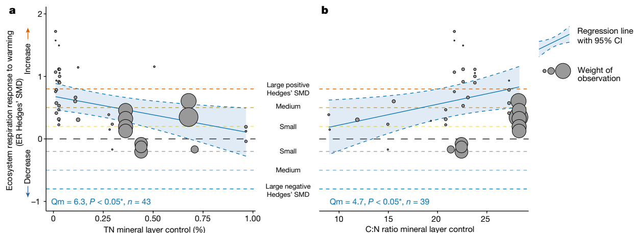
Fig. 5 | Context-dependencies in the ER response to warming. a, b , TN concentration (%) (a) and C:N ratio (b) of the mineral soil layer affected the ER response to experimental warming. The environmental drivers on the x-axis reflect mean values of measured soil conditions at the control plots of each experiment with available data. ER Hedges' SMDs for individual datasets are shown on the y-axis with grey bubbles, calculated as (mean ER of the warmed plots – mean of the control plots)/pooled standard deviation. Bubble size denotes the weight of the observation used in the metaregression quantified as the inverse of the square root of within-study variance, with larger bubbles indicating greater weights. The significant regression lines with 95% CI are
