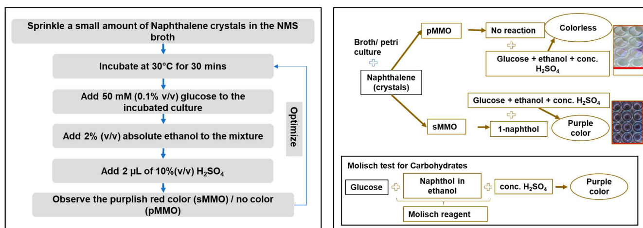
Figure 4. The optimization and working principle of naphthalene–Molisch assay.
