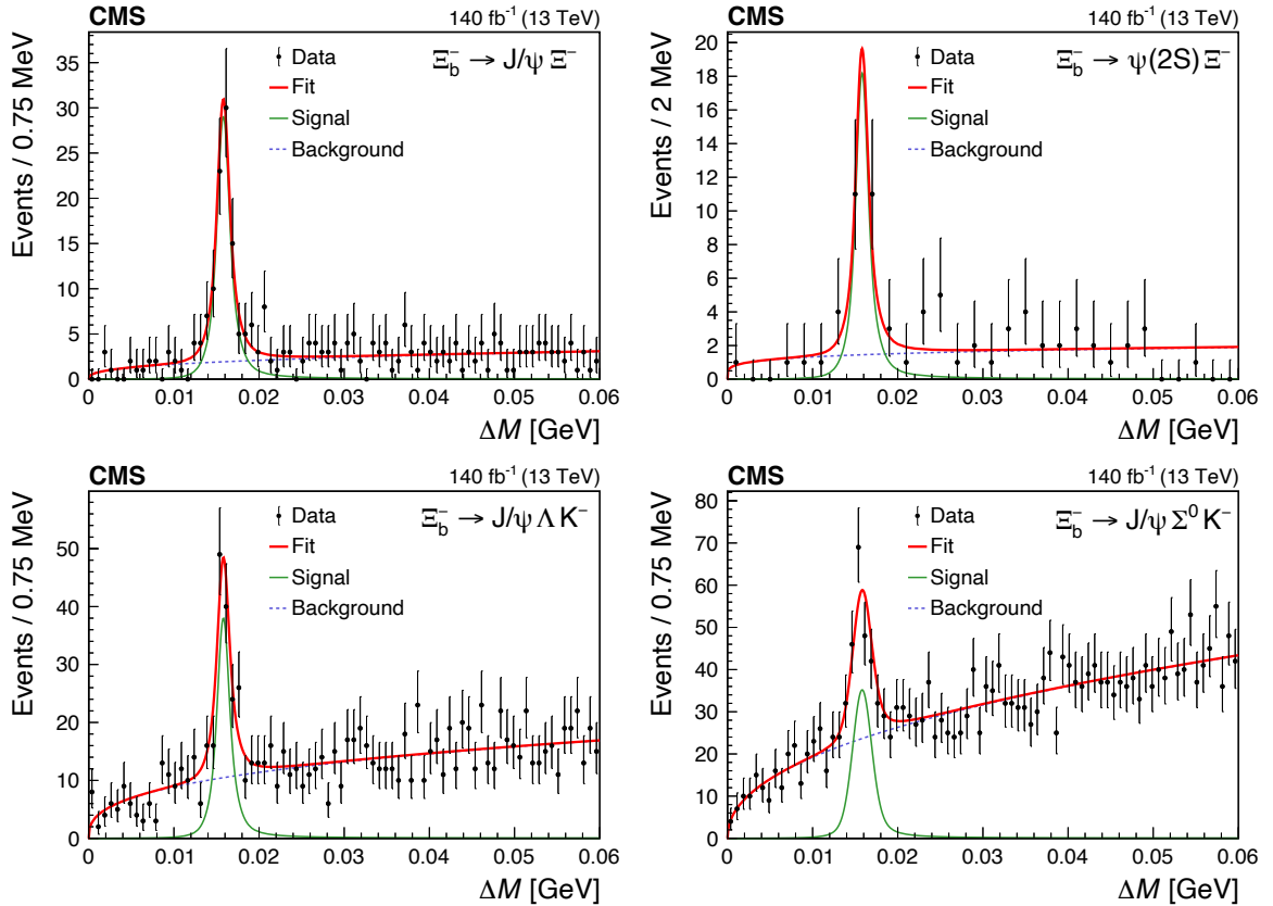
Figure 4: Results of the simultaneous fits to the \Delta M invariant mass distributions for the \Xi_b(5945)^0 candidates in the decay channels given in each plot. The points show the data, with the vertical bars representing the statistical uncertainty. The solid red curve displays the overall fit result, with the solid green and dashed blue curves showing the signal and background contributions, respectively.
