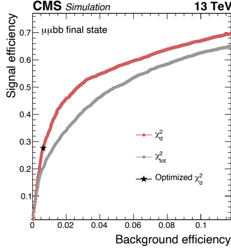
Figure 4: Signal ( m_{a_1} = 40 GeV) versus background efficiency for different thresholds on \chi_{\text{tot}}^2 (gray) and \chi_d^2 (red) variables. The black star indicates signal efficiency versus that of background for the optimized \chi_d^2 requirement.
