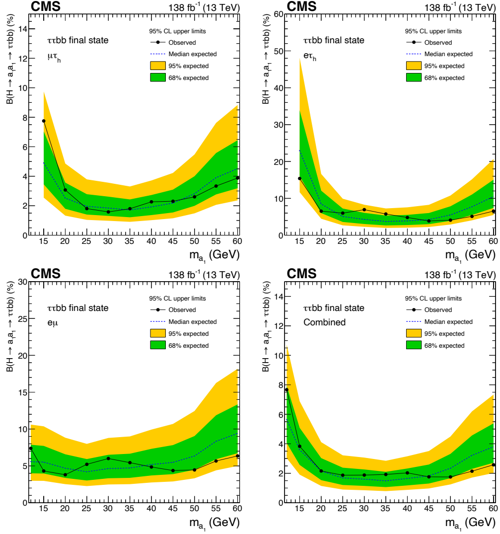
Figure 11: Observed and expected 95% CL exclusion limits on \mathcal{B}(H \rightarrow a_1 a_1 \rightarrow \tau\tau b\bar{b}) in percent, for the (upper left) \mu\tau_h , (upper right) e\tau_h , (lower left) e\mu channels, and (lower right) for the combination of all the channels.
