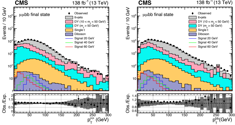
Figure 2: The p_T distributions of the (left) dimuon systems and (right) di-b-jet system. The uncertainty band in the lower panel represents the limited size of the simulated samples together with a 30% uncertainty in the low-mass DY cross section. Simulated samples are normalized to using the corresponding theoretical cross sections. To evaluate the normalization of the signal, SM Higgs boson cross sections are multiplied by the \mathcal{B}(a_1 a_1 \rightarrow \mu\mu bb) value that is calculated in the Type III model with \tan\beta = 2 .
