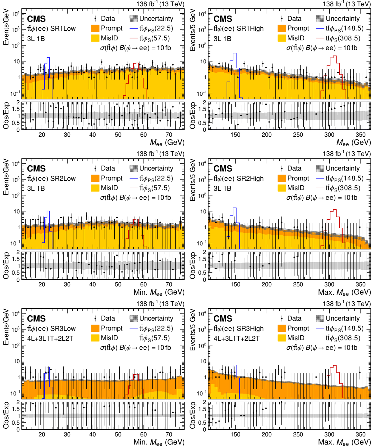
Figure 5: Dilepton mass spectra for the t\bar{t}\phi(ee) SR1 (upper), SR2 (middle), and SR3 (lower) event selections for the combined 2016–2018 data set. The low (high) mass spectra are shown on the left (right). The lower panel shows the ratio of observed events to the total expected SM background prediction (Obs/Exp), and the gray band represents the sum of statistical and systematic uncertainties in the background prediction. The expected background distributions and the uncertainties are shown after the data is fit under the background-only hypothesis. For illustration, two example signal hypotheses for the production and decay of a scalar and a pseudoscalar \phi boson are shown, and their masses (in units of GeV) are indicated in the legend. The signals are normalized to the product of the cross section and branching fraction of 10 fb.
