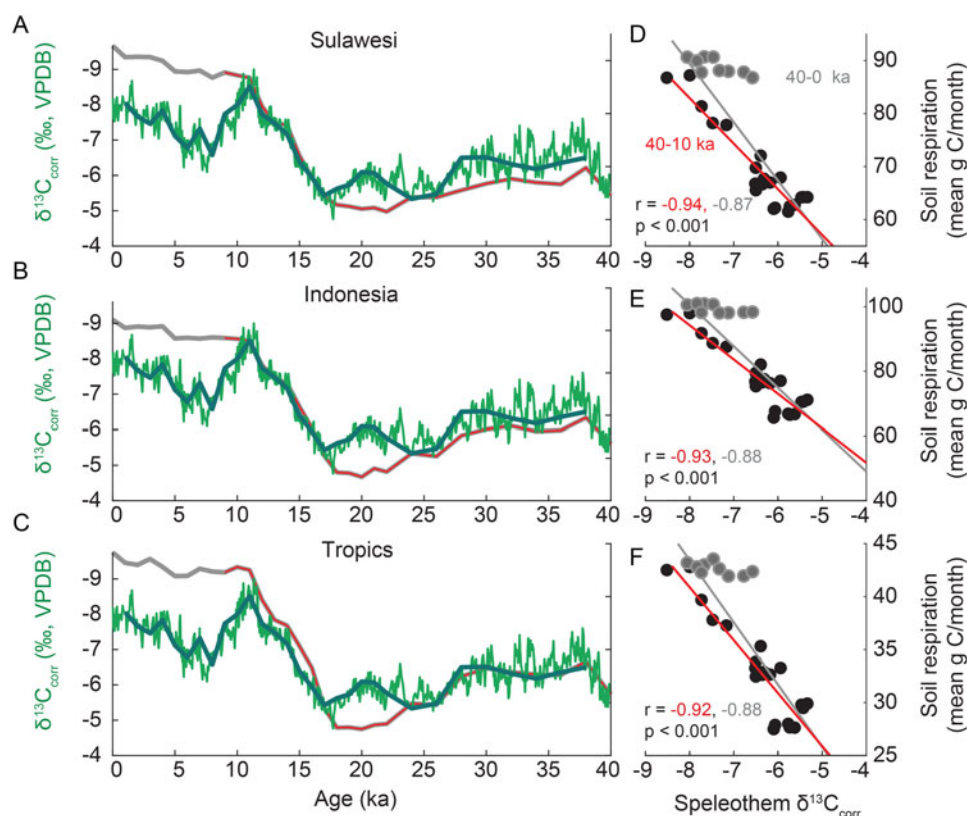
Figure 8. Comparison of modelled mean soil respiration and Sulawesi stalagmite \delta^{13}\text{C} . (A–C) Time series of modelled mean soil respiration for the grid points corresponding to Sulawesi, Indonesia, and tropics ( \pm 30^\circ ). Sulawesi stalagmite \delta^{13}\text{C} is plotted on each graph for reference (the bold green curve has been resampled to match the 1 ka model resolution). (D–F) Relationships between modelled mean soil respiration and stalagmite \delta^{13}\text{C} , with regression statistics. Results for the glacial and deglacial periods only (40–10 ka) are in red; those for the full record (40–0 ka) are in grey.
