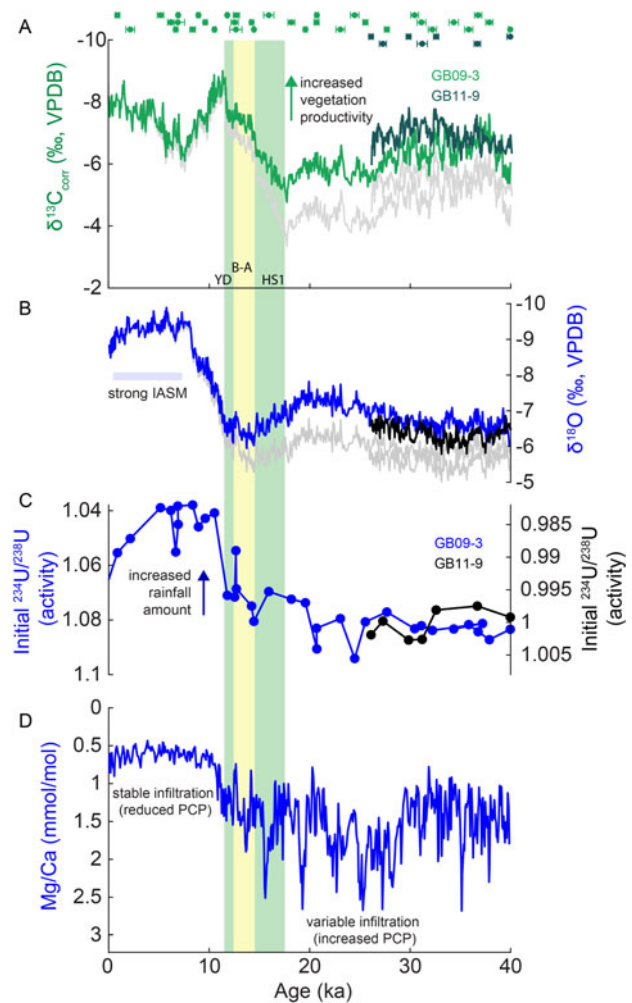
Figure 3. Stalagmite \delta^{13}\text{C} , \delta^{18}\text{O} , initial ^{234}\text{U}/^{238}\text{U} , and Mg/Ca records for Sulawesi over the last 40 ka. (A) \delta^{13}\text{C} for GB09-3 and GB11-9 corrected for the effect of atmospheric CO 2 on carbon isotope fractionation in C 3 plants (Breecker, 2017). Uncorrected \delta^{13}\text{C} is shown in grey. The large deglacial \delta^{13}\text{C} transition (green shading) encompasses two abrupt negative excursions at ~14.7–14.5 ka and 11.7–11.6 ka that mark the terminations of Heinrich stadial 1 (HS1) and the Younger Dryas (YD), respectively. The Bolling-Allerød (B-A) is also shown (yellow). (B) \delta^{18}\text{O} for GB09-3 and GB11-9 corrected for the effect of ice volume (Krause et al. , 2019). Uncorrected \delta^{18}\text{O} shown in grey. (C) Initial ^{234}\text{U}/^{238}\text{U} records for GB09-3 and GB11-9. (D) Mg/Ca record for GB09-3. The late-deglacial transition to lower values in all three hydroclimate proxies is interpreted as an increase in rainfall amount and a strengthened Indo-Australian summer monsoon (IASM). Initial ^{234}\text{U}/^{238}\text{U} is influenced by drip-water flow pathways; thus, coeval stalagmites are unlikely to share the same values and are therefore plotted on separate scales. ^{230}\text{Th} dates with 2\sigma errors are shown at the top of the figure. PCP, prior calcite precipitation.
