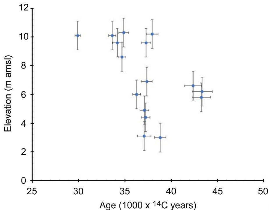
Figure 7. Age-elevation relationship of radiocarbon dated shells within raised beach deposits at Kai-no-hama beach, East Ongul Island, Lutzow-Holm Bay, East Antarctica. Age and elevations from Miura et al. (1998).
