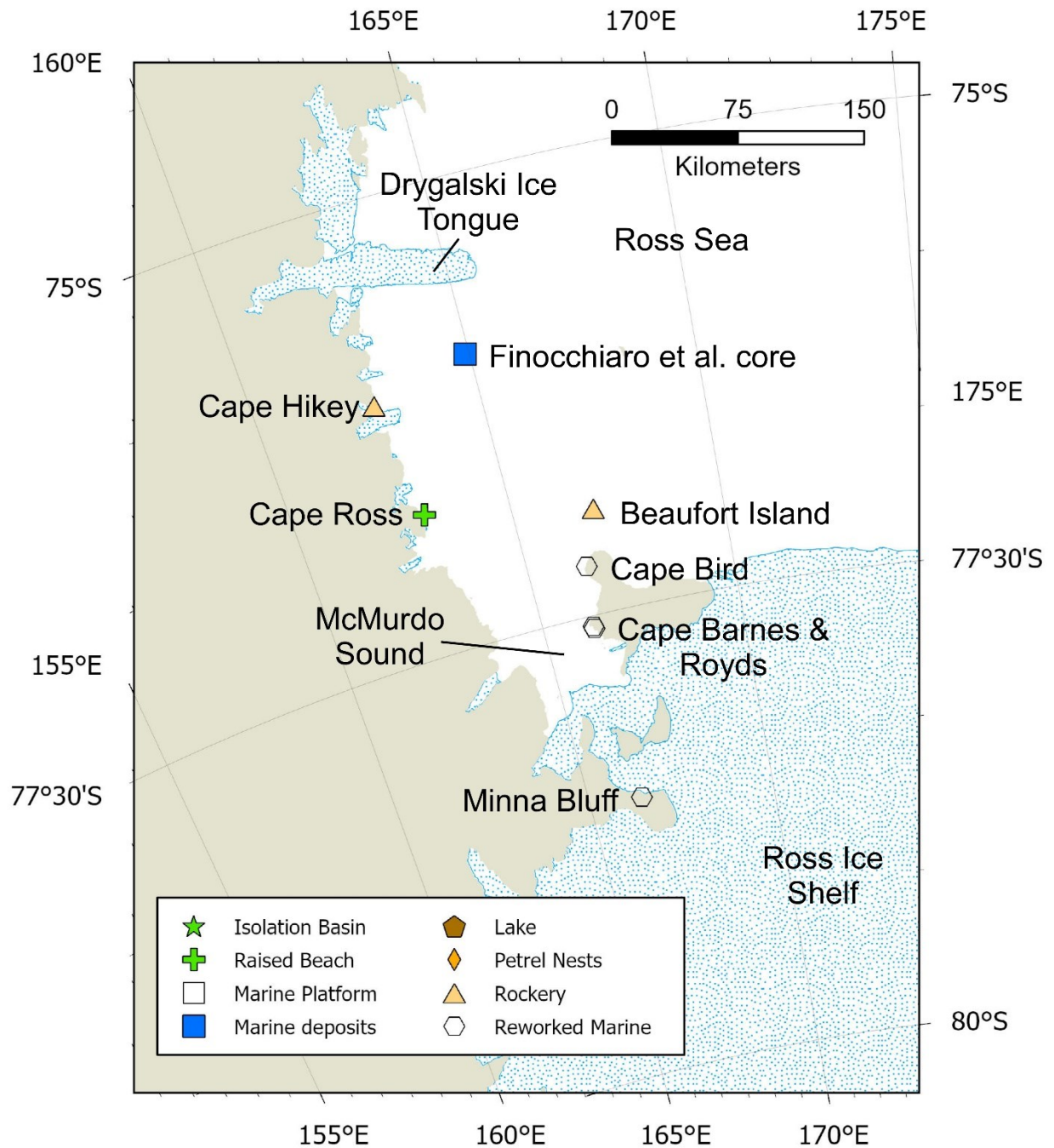
Figure 13. Map showing the general locations of Late Pleistocene deposits mentioned in the Ross Sea. See Figure 1 for general location.
