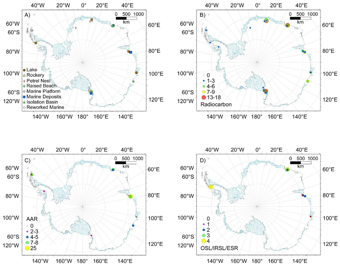
Figure 2. Distribution of Late Pleistocene relative sea-level constraints based on indicype (a), radiocarbon dating (b), amino acid racemization (c), and luminescence techniques (d).
