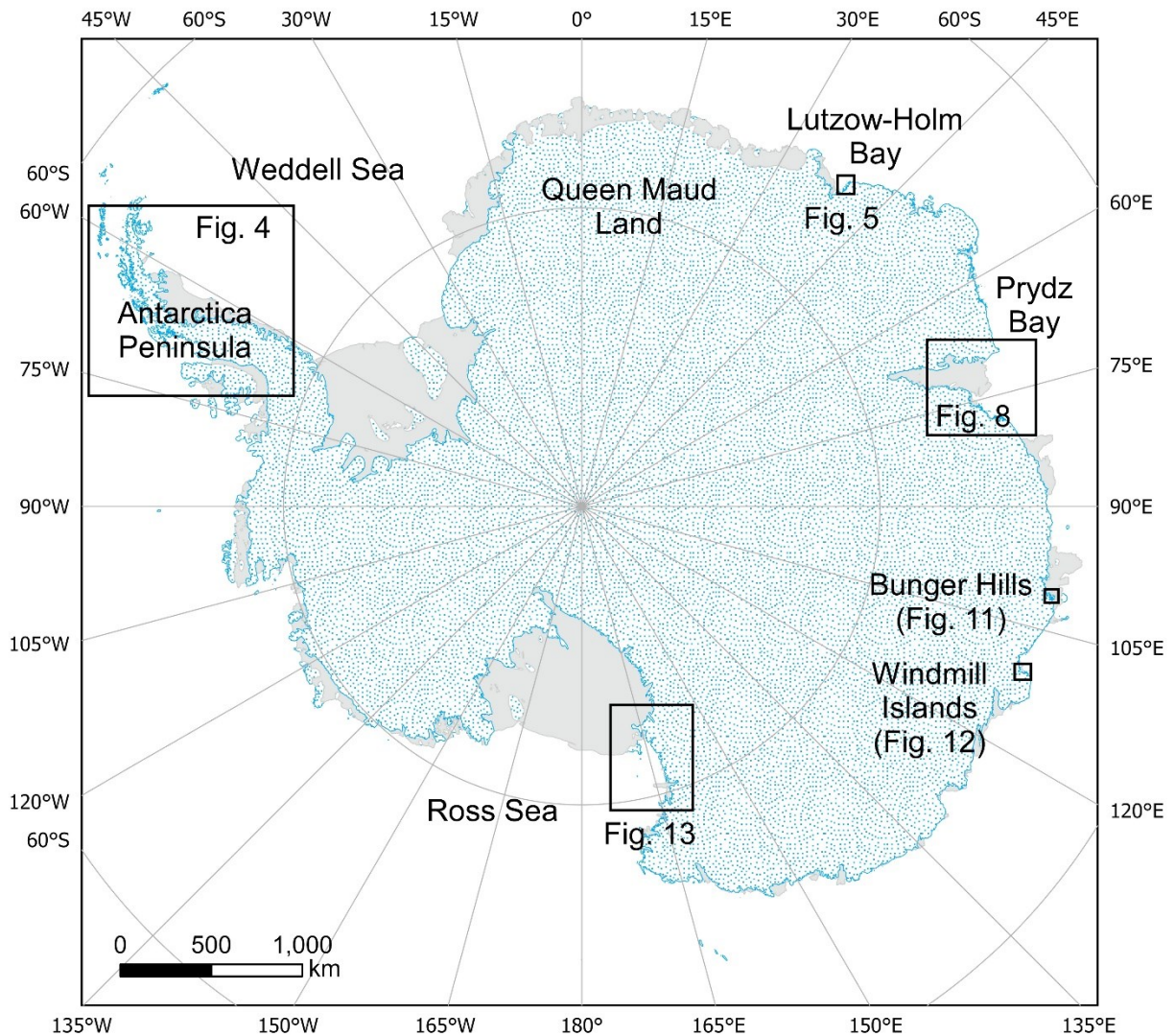
Figure 1. Map of Antarctica showing the major zones of Antarctica and the location of sites mentioned in the text
