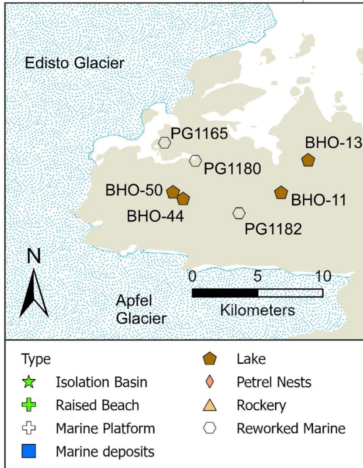
Figure 11. Map showing the locations of Late Pleistocene ages obtained in the Bunger Hills. Samples labeled “BHO” are OSL ages from kettle and glacial lake shorelines collected by Gore et al. (2000). The PG samples are from sediment cores from lake basins collected by Melles et al. (1997) and Kulbe (1997). See Figure 1 for general location.
