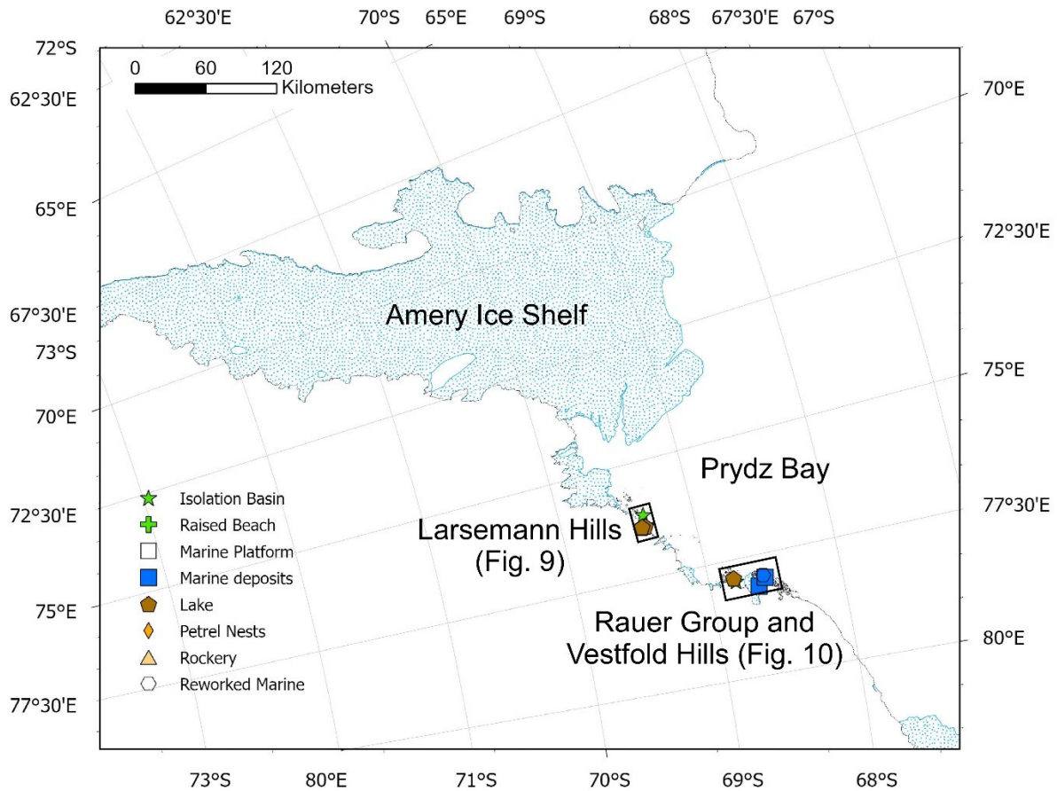
Figure 8. Map showing the general locations of the Larsemann Hills, Vestfold Hills, and Rauer Group within Prydz-Bay, East Antarctica.
