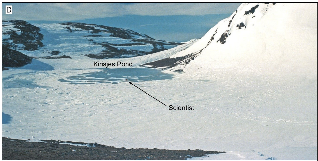
Figure 3. Photographs of Late Pleistocene features from across Antarctica. A. Holocene strandplain and
