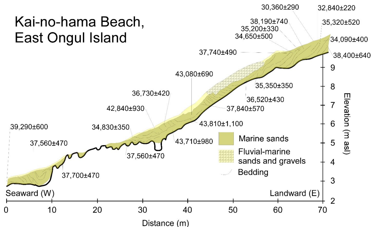
Figure 6. Profile and stratigraphic description of the trench at Kai-no-hama, East Ongul Island. Ages shown are based on radiocarbon dating in ^{14}\text{C} years. Adapted from Muira et al. (1998a) and Takada et al. (2003).
