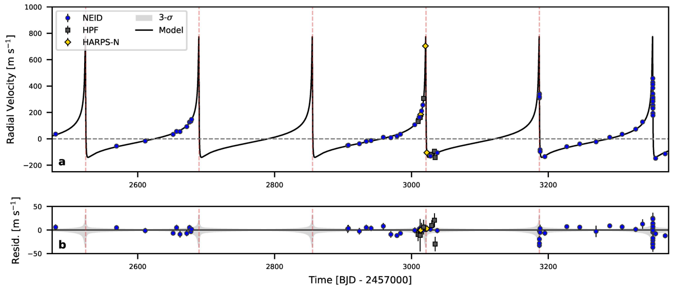
Extended Data Fig. 3 | RV time series for TIC241249530. a. RV measurements from NEID (blue), HPF (black) and HARPS-N (gold) and best-fit orbit model (black curve). b. Residuals to the RV orbit fit. Vertical red lines in both panels mark the predicted transit times. The grey-shaded region bounds the 3 \sigma confidence intervals for the fit. The horizontal axis is in units of days relative to Barycentric Julian Date (BJD) 2457000. Error bars on individual points represent 1 \sigma measurement uncertainties.
