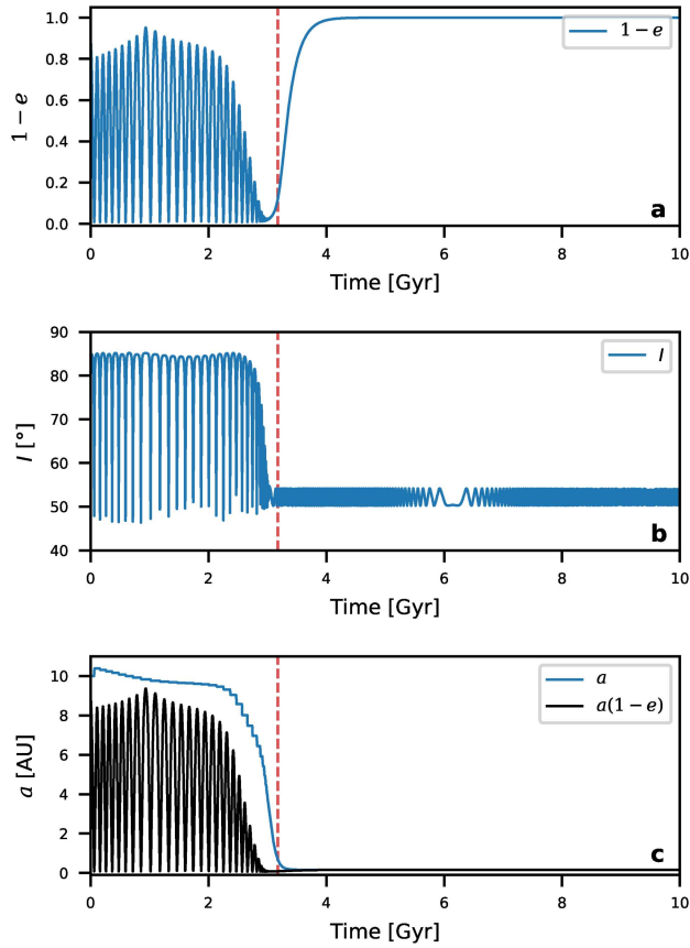
Extended Data Fig. 6 | Simulated evolution of the orbit of TIC 241249530 b resulting from high-eccentricity migration driven by vZLK oscillations.
