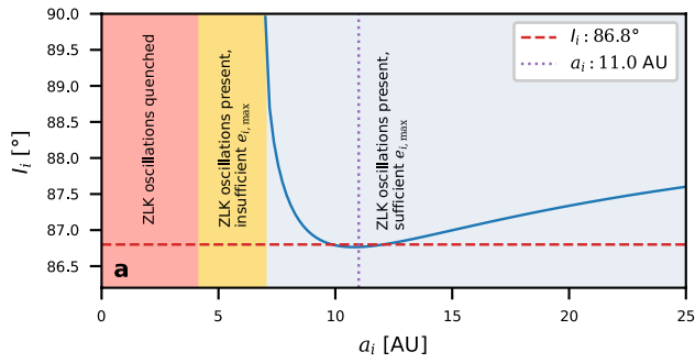
Extended Data Fig. 5 | Constraints on the parameters of the first vZLK oscillation for TIC 241249530 b. a, Constraints on initial inclination.
