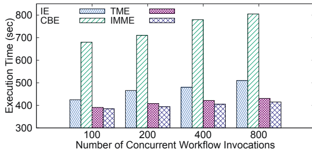
Fig. 11: Impact of our runtime on execution time on an 8-node cluster.
